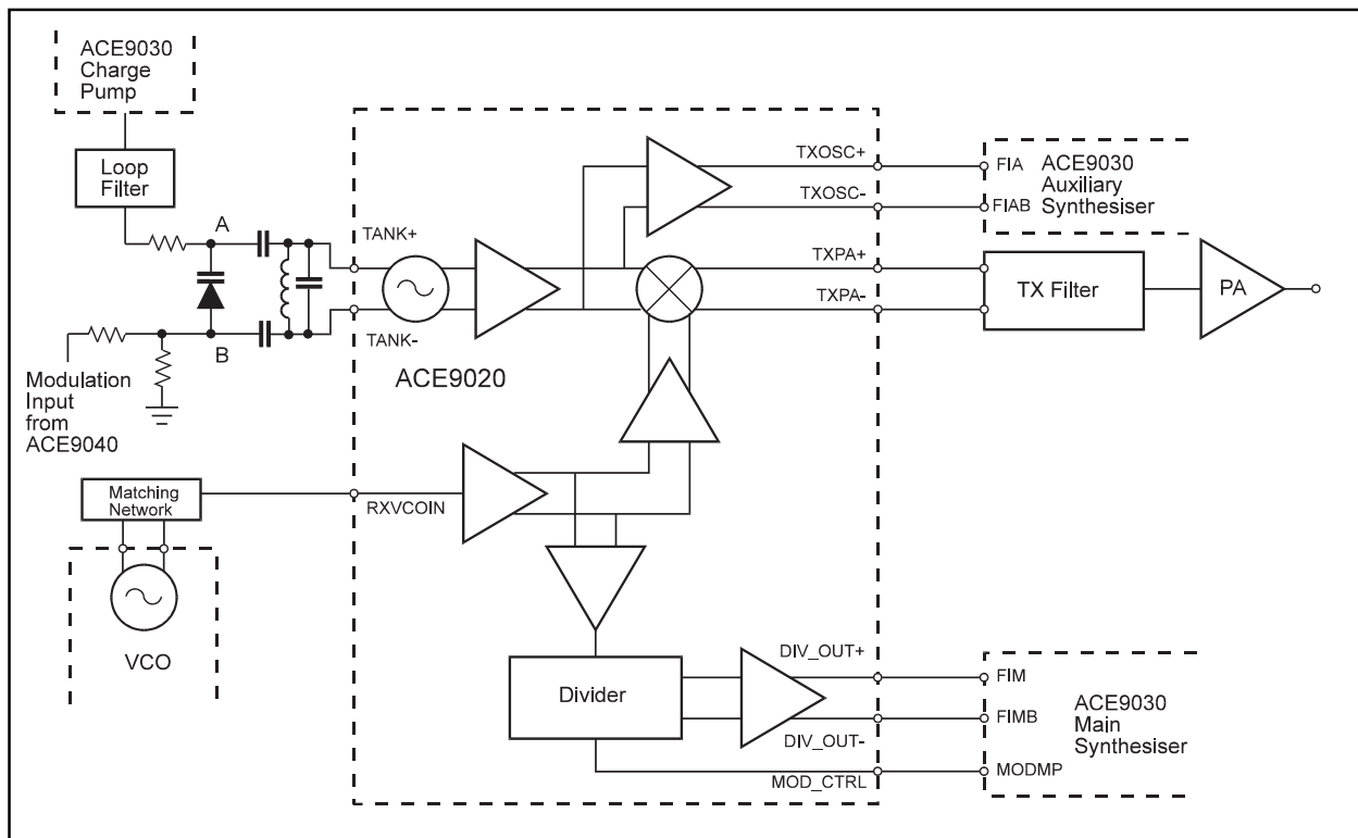
Figure 4 - Application Diagram
