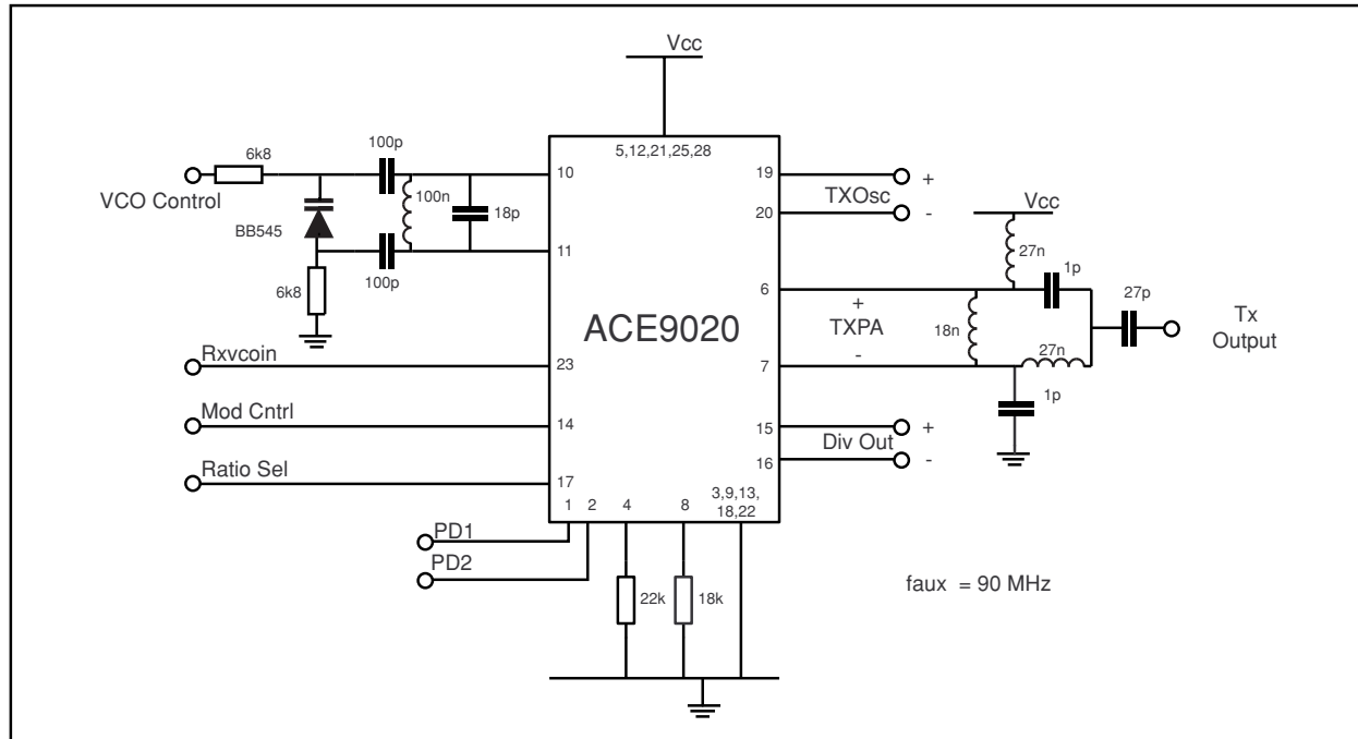
Figure 3 - ACE9020 Test circuit
