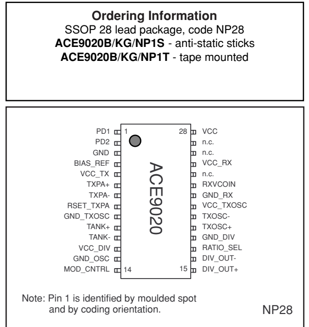
Figure 1 - Pin connections - top view
