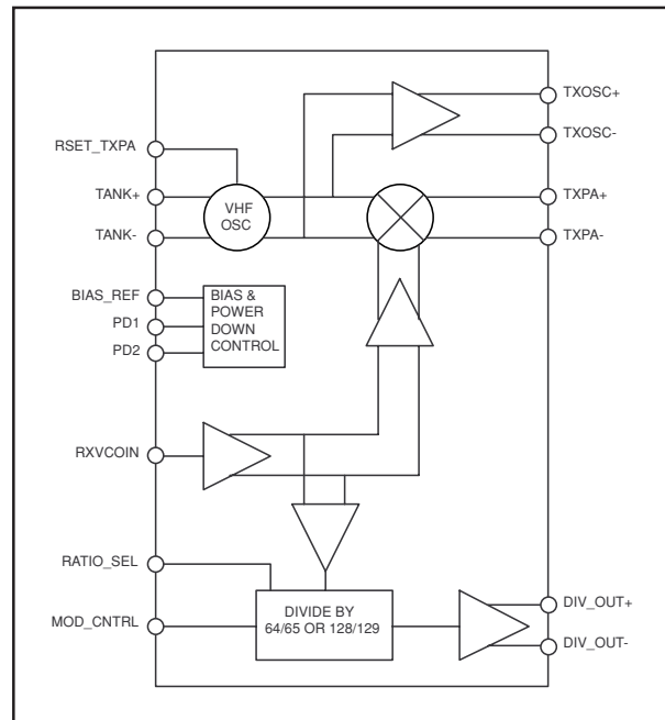
Figure 2 - ACE9020 simplified block diagram
