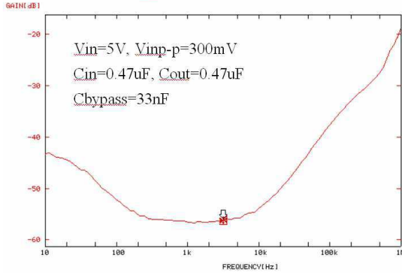
PSRR vs Frequency (Load=1mA)
