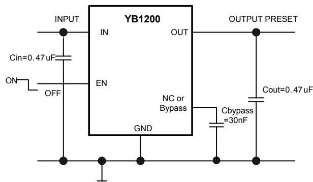
Figure 1-1. SC-70 application circuit
