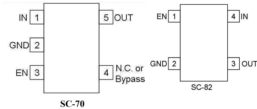
Figure 2. Pin configuration
