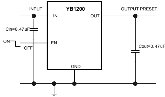
Figure 1-2. SC-82 application circuit
