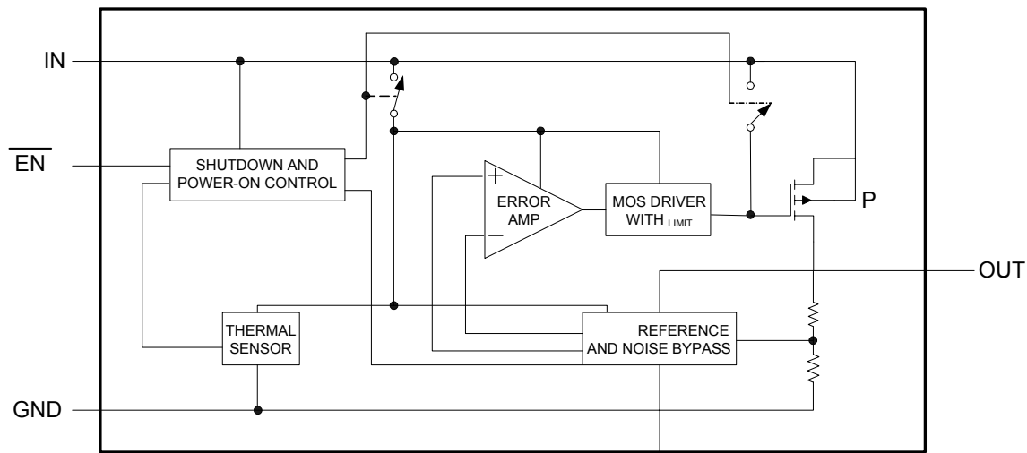
Figure 3. Block Diagram
