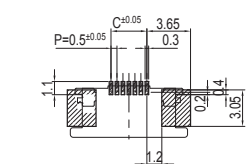
PCB LAYOUT (05003HR-00A01)
