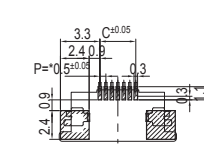
PCB LAYOUT (05003HR-00A02)
