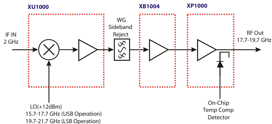
Mimix Broadband MMIC-based 17.0-24.0 GHz Transmitter Block Diagram (Changing LO and IF frequencies as required allows design to operate as high as 24 GHz)
