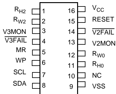
X40237 16 Pin SOIC
