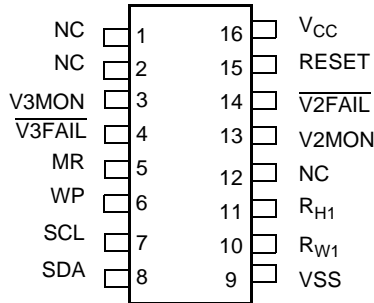
X40233 16 Pin SOIC
