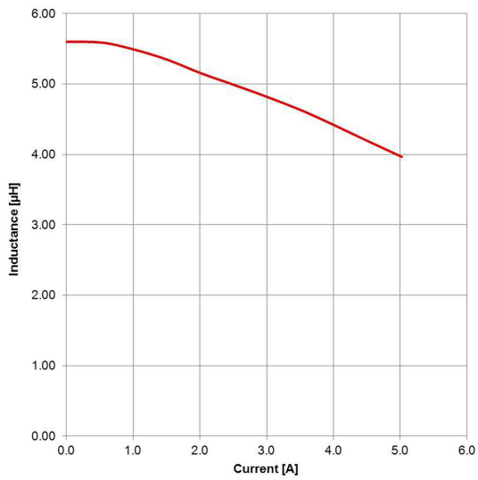
F Typical Inductance vs. Current Characteristics:
