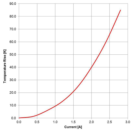
F Typical Temperature rise vs. Current Characteristics:
