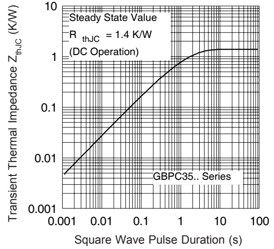
Fig. 12 - Thermal Impedance Z_{thJC} Characteristic
