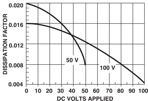
DISSIPATION FACTOR VS. VOLTAGE
