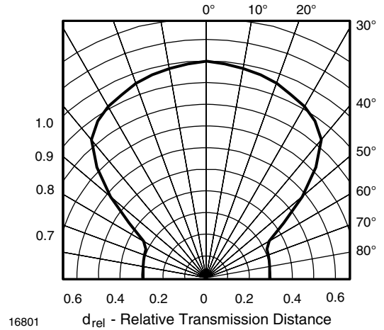
Fig. 12 - Directivity
