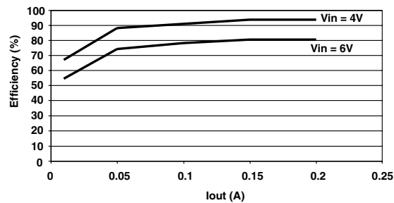
Efficiency Vs. Iout*
