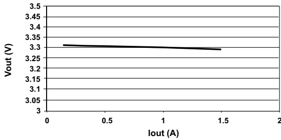
Vout Vs. Iout* Vin = 3.6V
