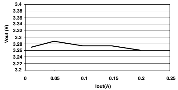
Vout Vs. Iout* Vin = 6V
