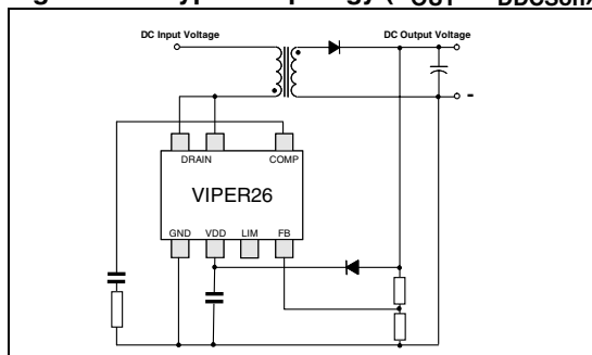
Figure 1. Typical topology ( V_{OUT} \leq V_{DCCSon} )
