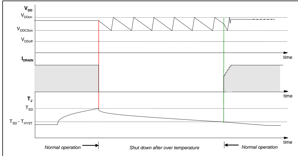
Figure 16. Thermal shutdown
