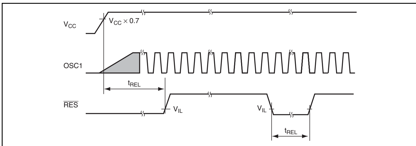
Figure 20.2 \overline{\text{RES}} Low Width Timing
