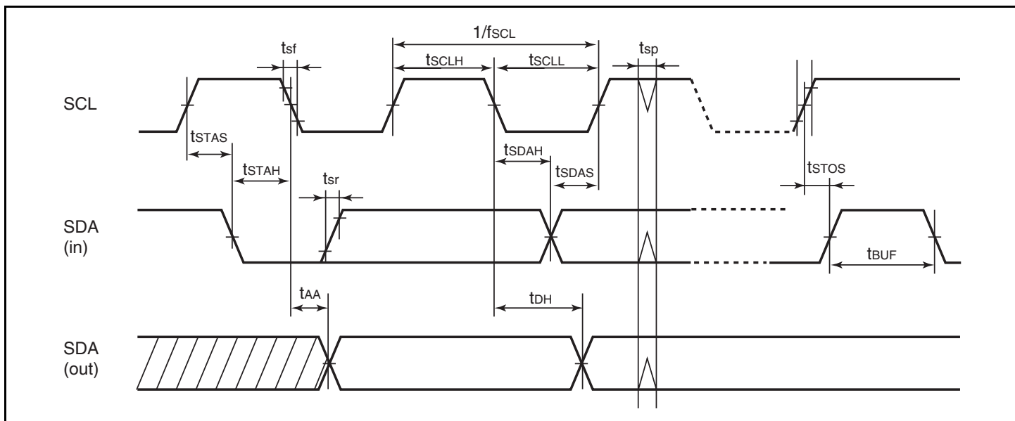
Figure 20.7 EEPROM Bus Timing
