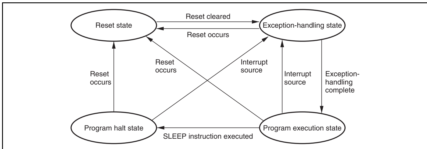
Figure 2.12 State Transitions
