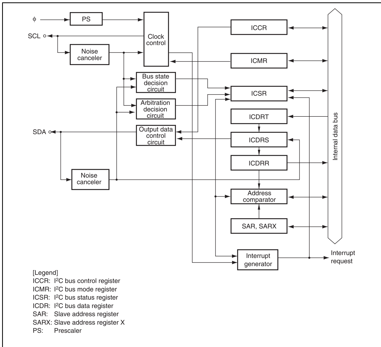
Figure 15.1 Block Diagram of I 2 C Bus Interface
