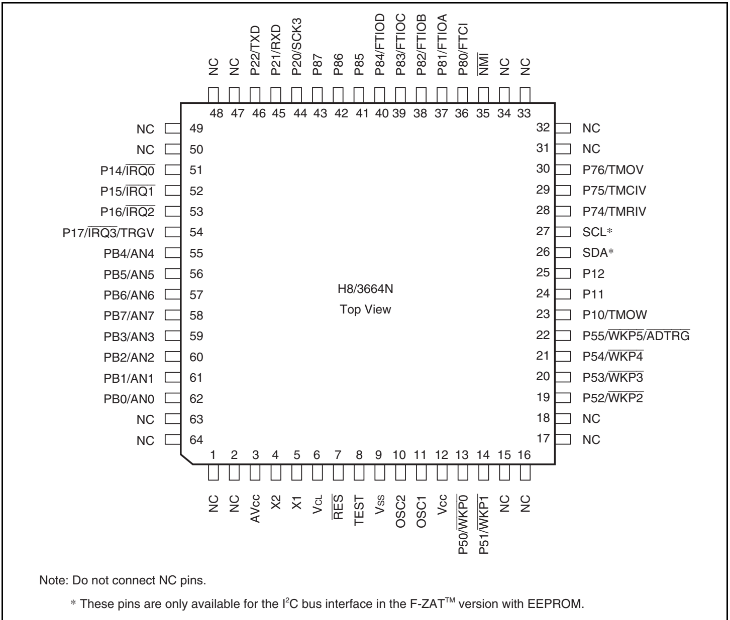
Figure 1.6 Pin Arrangement of H8/3664N of F-ZAT™ Version with EEPROM (FP-64E)
