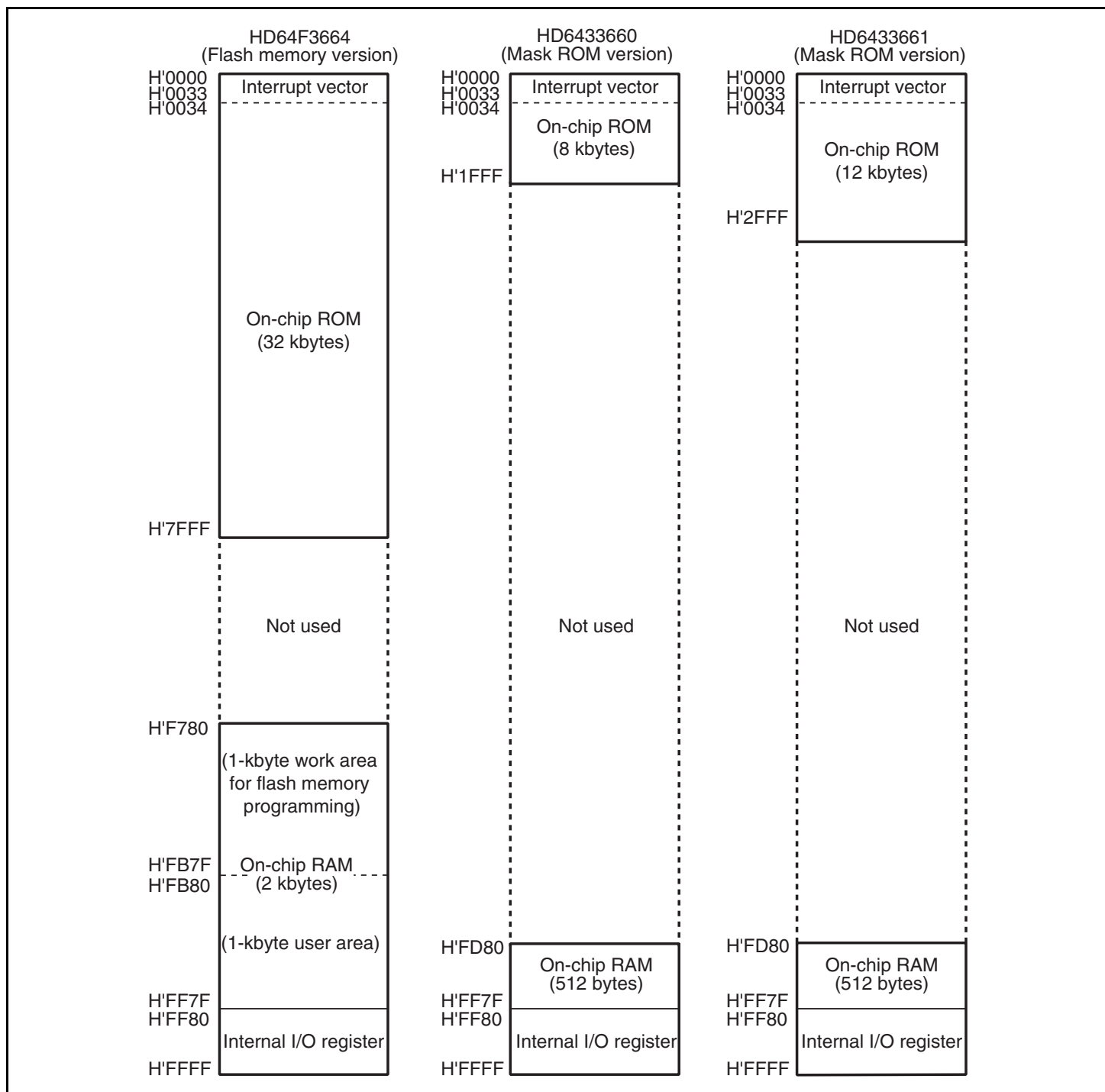
Figure 2.1 Memory Map (1)
