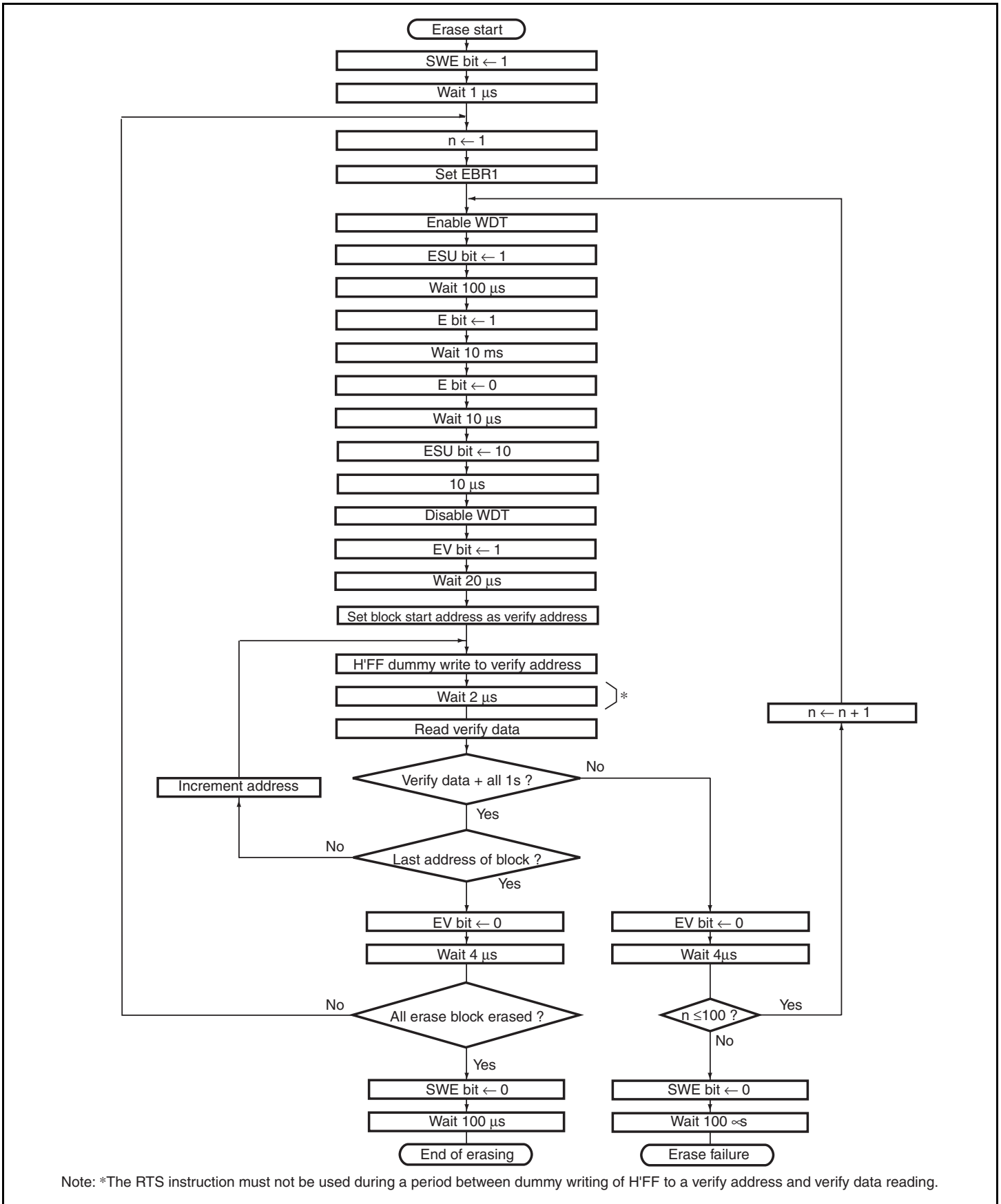
Figure 7.4 Erase/Eraser-Verify Flowchart
