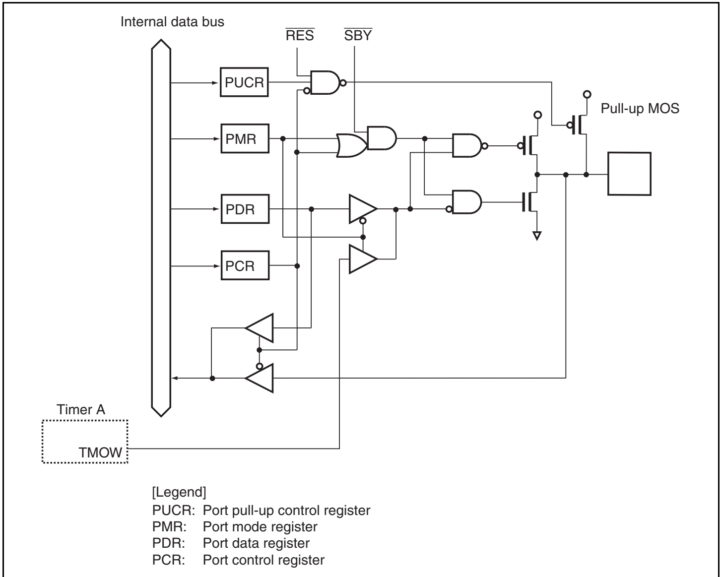
Figure B.4 Port 1 Block Diagram (P10)
