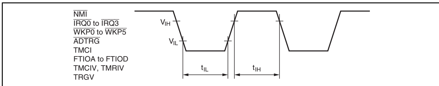
Figure 20.3 Input Timing
