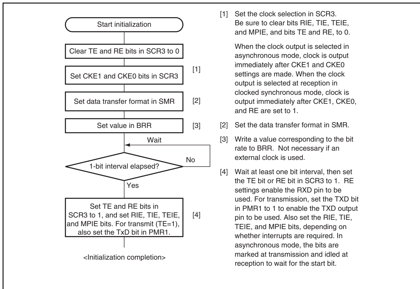
Figure 14.4 Sample SCI3 Initialization Flowchart
