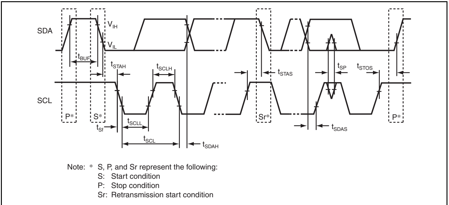
Figure 20.4 I 2 C Bus Interface Input/Output Timing
