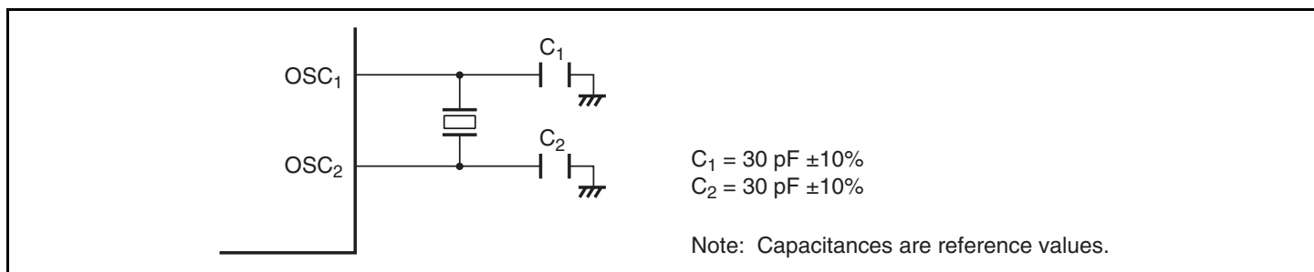
Figure 5.5 Typical Connection to Ceramic Resonator
