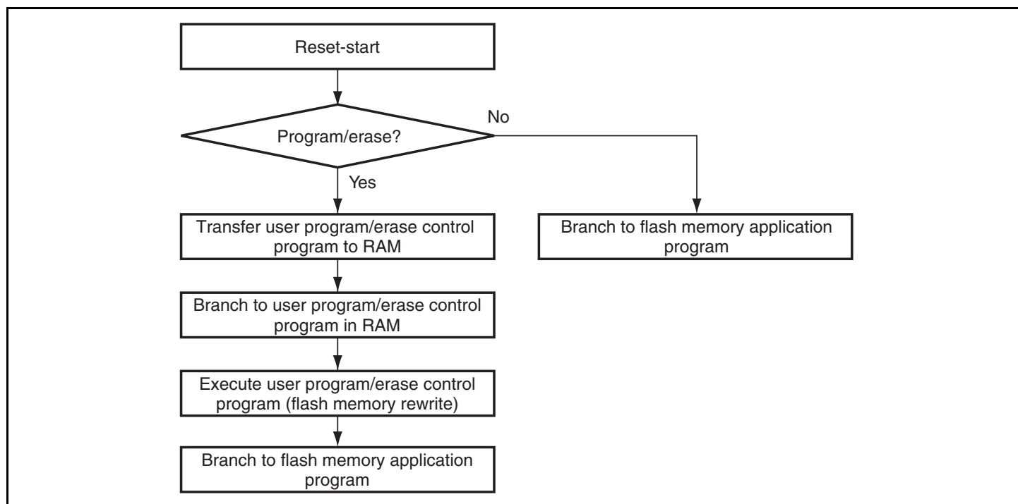
Figure 7.2 Programming/Erasing Flowchart Example in User Program Mode
