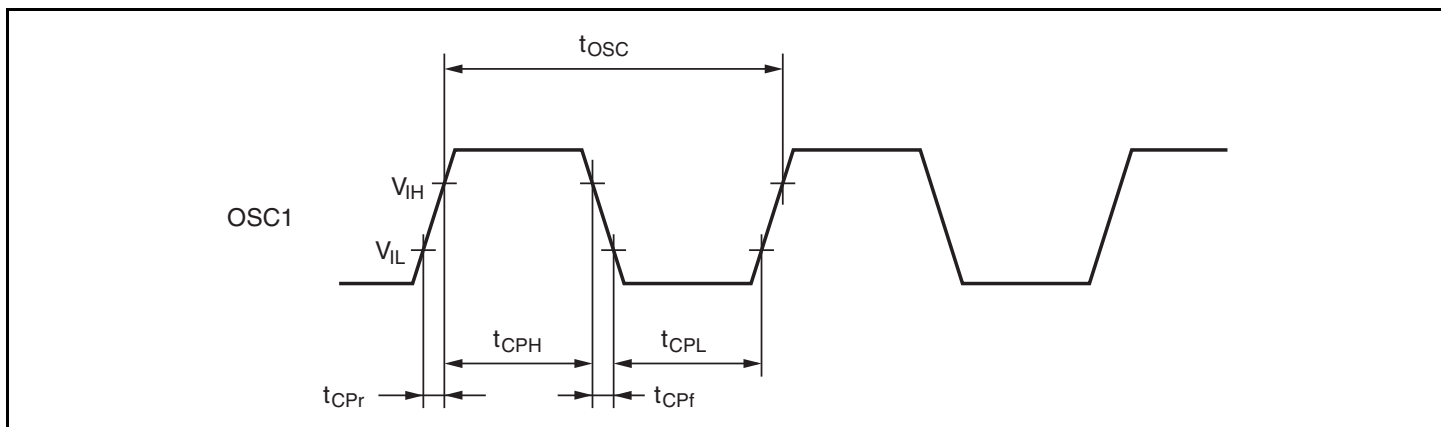
Figure 20.1 System Clock Input Timing
