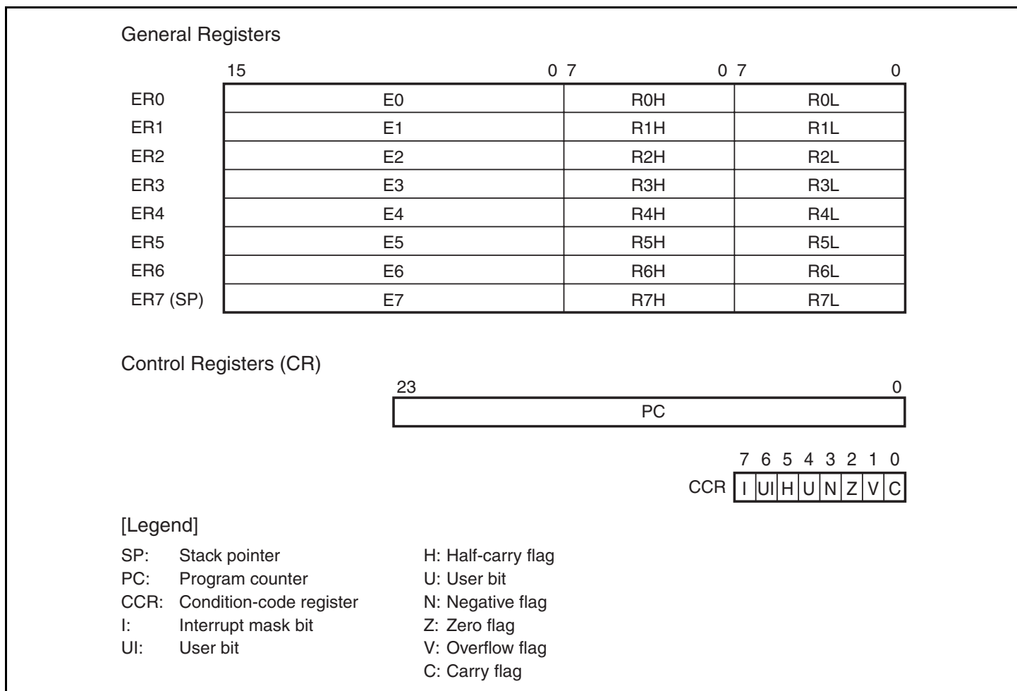
Figure 2.2 CPU Registers
