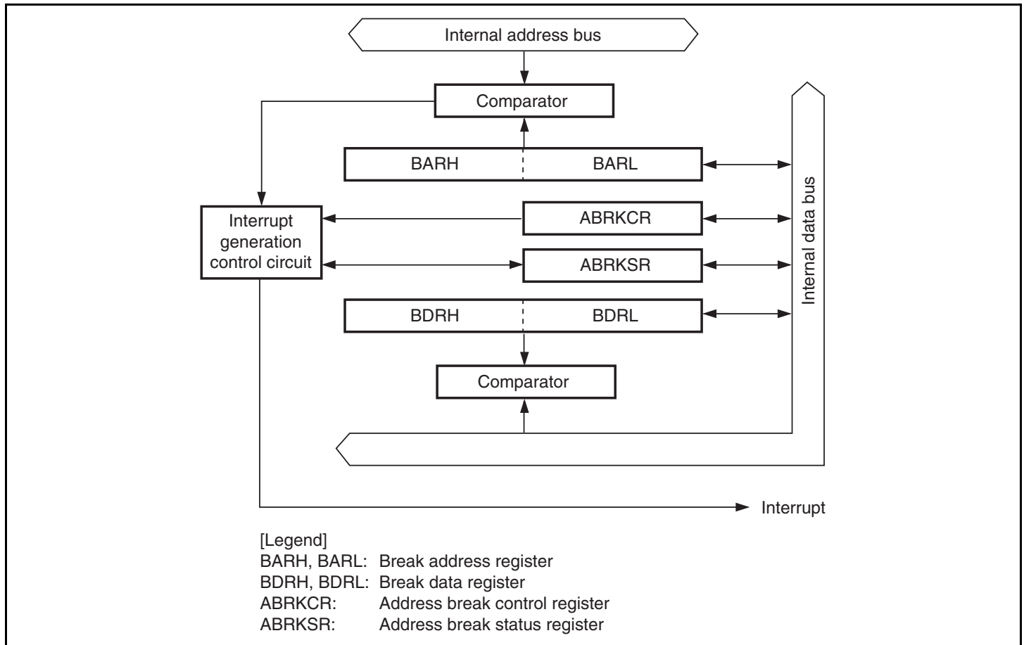
Figure 4.1 Block Diagram of Address Break
