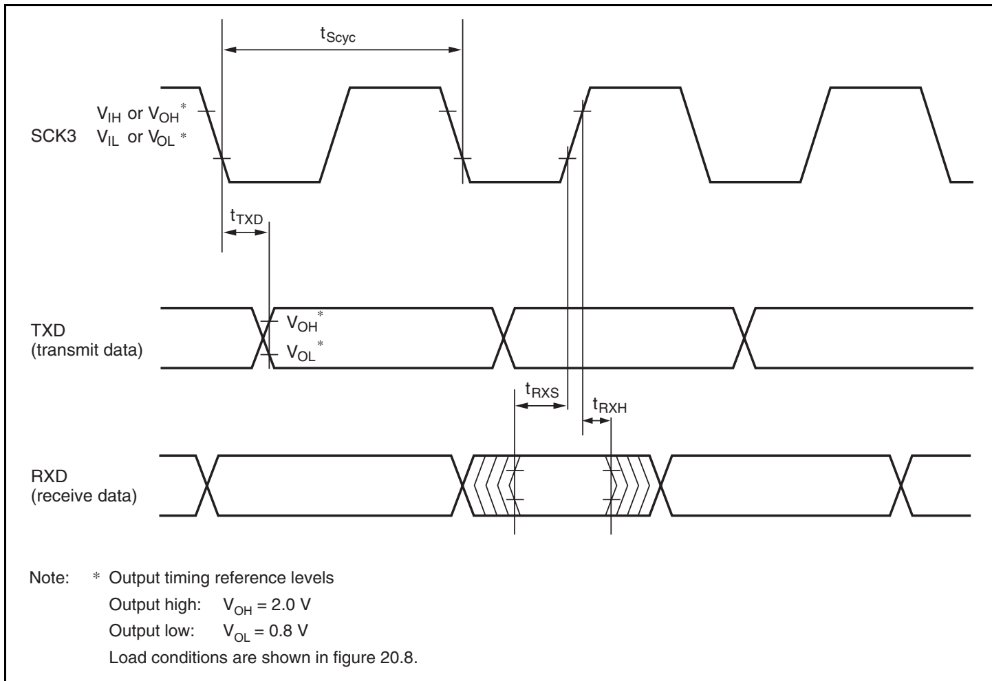
Figure 20.6 SCI3 Input/Output Timing in Clocked Synchronous Mode
