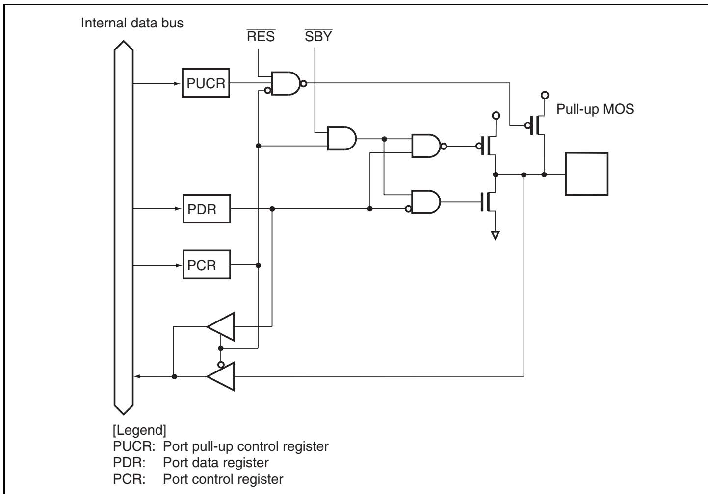
Figure B.3 Port 1 Block Diagram (P12, P11)
