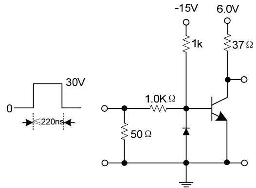
Saturated Turn-Off Switching Time
