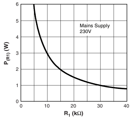
Figure 6-12. Power Dissipation of R_1
