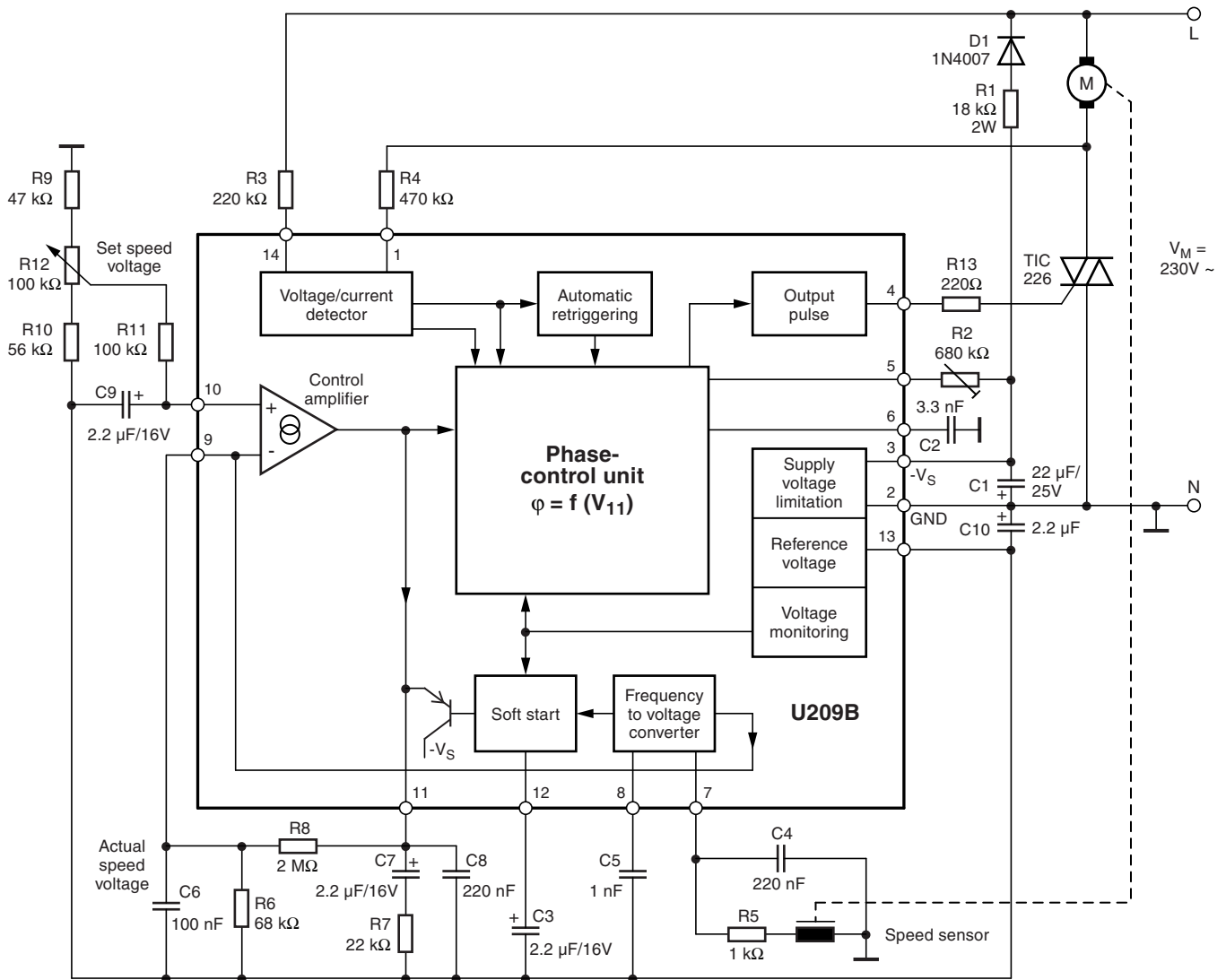
Figure 1-2. Block Diagram with Typical Circuitry for Speed Regulation
