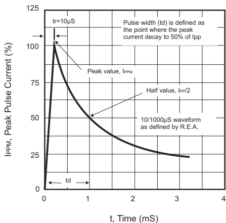
Fig.5 Pulse Waveform
