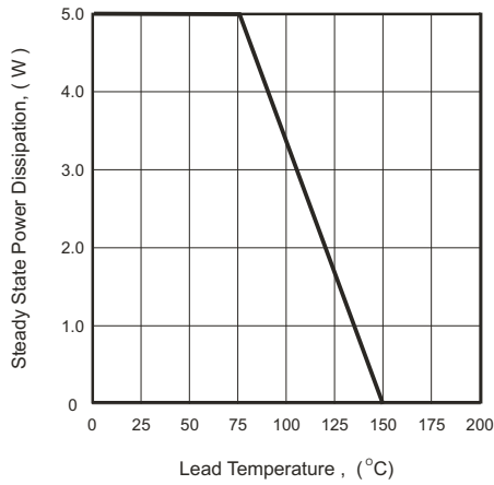
Fig.3 Steady State Power Derating Curve
