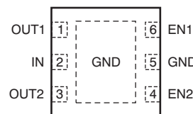
TPS718xx, TPS719xx DRVP package 2mm \times 2mm SON-6 (TopView)
