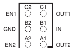
TPS718xx, TPS719xx YZCP package 6-BALL WCSP (TopView)
