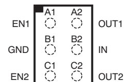
TPS718Axx, TPS719Axx YZCP package 6-BALL WCSP (TopView)
