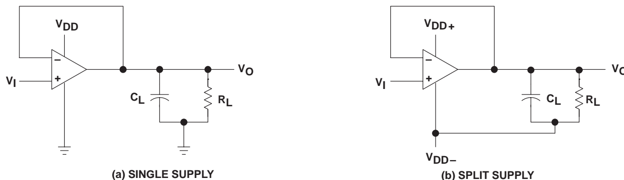
Figure 35. Unity-Gain Amplifier
