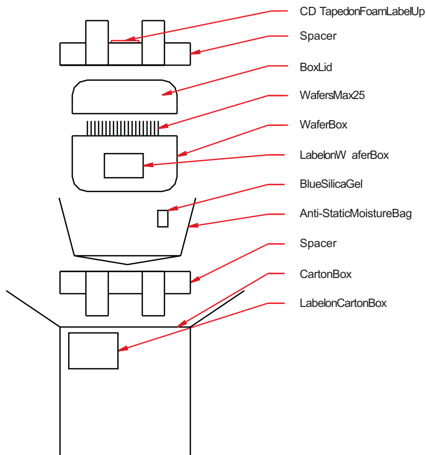
Figure 3-5. Packing of Wafers
