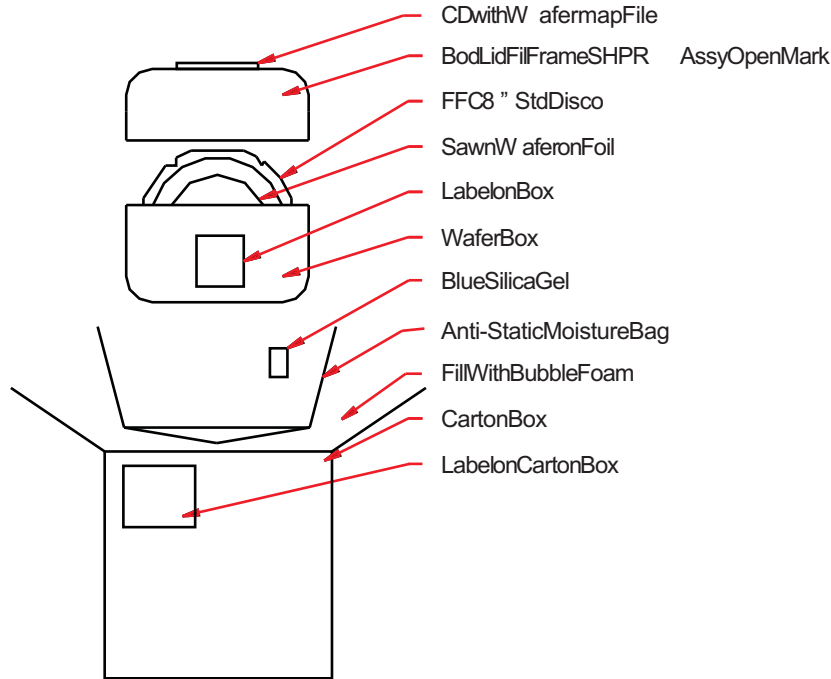
Figure 3-6. Packing of Sawn Wafers (Multi)
