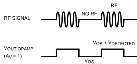
Figure 8. Offset Voltage Variation Due to an Interfering RF Signal
