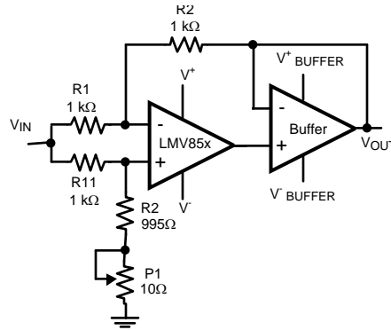
Figure 5. AC CMRR Measurement Setup
