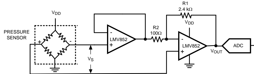
Figure 11. Pressure Sensor Application
