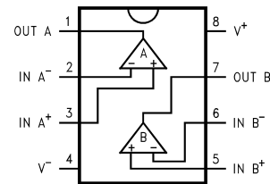
Figure 3. 8-Pin MSOP (Top View)
