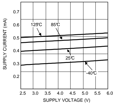
Supply Current vs. Supply Voltage Quad LMV854
