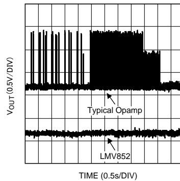
Figure 10. Comparing EMI Robustness
