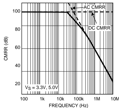
Figure 6. CMRR Curve
