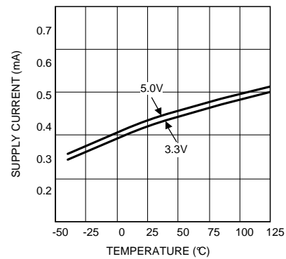
Supply Current vs. Temperature Single LMV851
