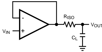
Figure 7. Isolating Capacitive Load
