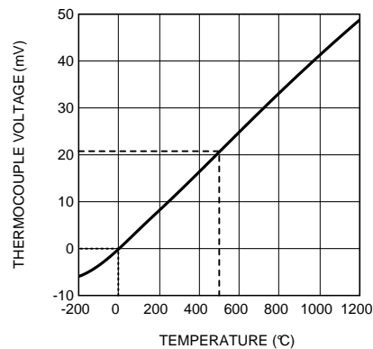
Figure 12. K-Type Thermocouple Response
