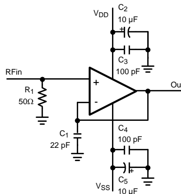
Figure 9. Circuit for Coupling the RF Signal to IN +
