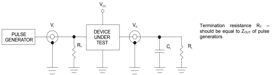
Figure 2. Test Circuit
