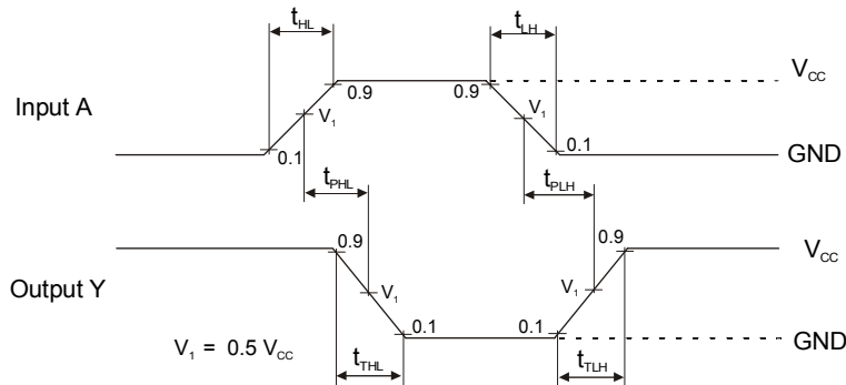
Figure 1. Switching Waveforms
