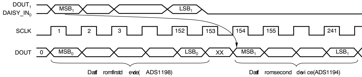
Figure 37. Daisy-Chain Timing
