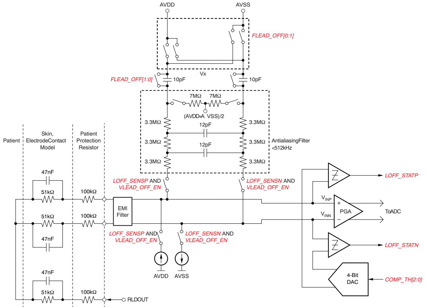
Figure 48. Lead-Off Detection
