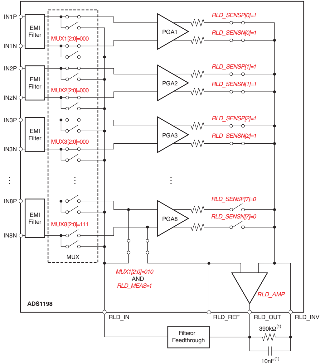
Figure 43. RLDOUT Signal Configured to be Read Back by Channel 8
