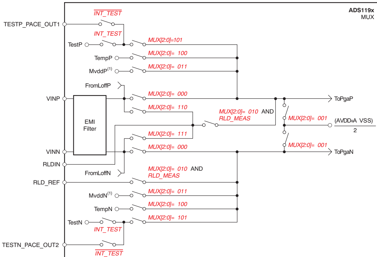
Figure 15. Input Multiplexer Block for One Channel
