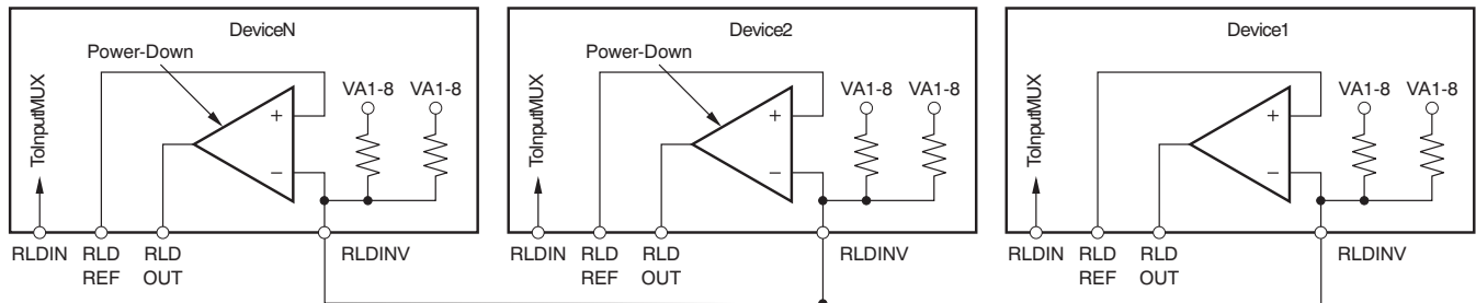
Figure 52. RLD Connection for Multiple Devices
