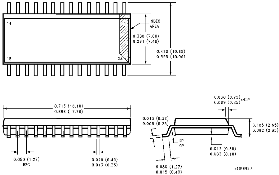
Small Outline Molded Dual-In-Line Package (M) Order Number COP881C-XXX/WM, COP981C-XXX/WM, COP681C-XXX/WM or COP981CH-XXX/WM NS Package Number M28B
