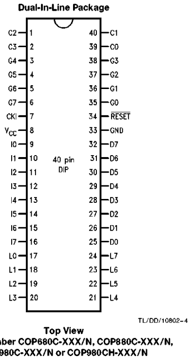
FIGURE 3. Connection Diagrams
