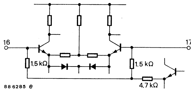
Figure 9. Pin 16, 17: IF input sound carrier
