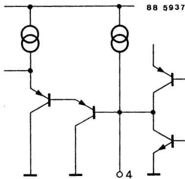
Figure 4. Pin 4: AGC storage capacitor
