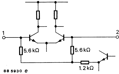
Figure 2. Pin 1, 2: IF input vision carrier
