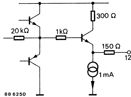
Figure 6. Pin 12: AF output 2
