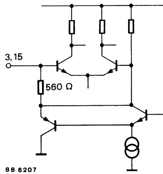
Figure 3. Pin 3 (15): Intercarrier input Pin 3 = 5.74 MHz, Pin 15 = 5.5 MHz
