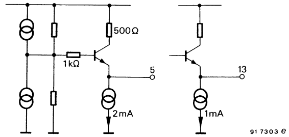
Figure 5. Pin 5 (13): Intercarrier output Pin 5 = 5.74 MHz, Pin 13 = 5.5 MHz
