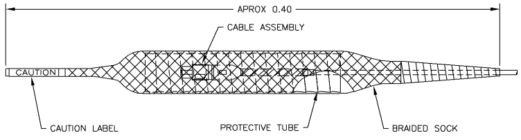
PROTECTIVE COVER BOTTOM END
