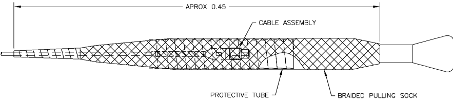
PULLING SOCK TOP END
