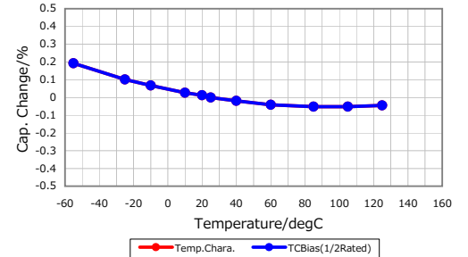
Temperature Characteristic
