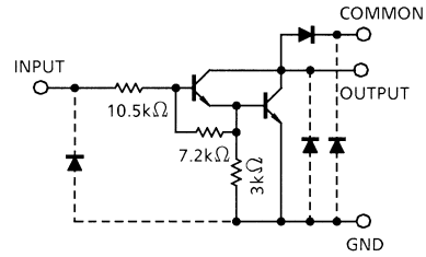
TD62004APG/AFG
