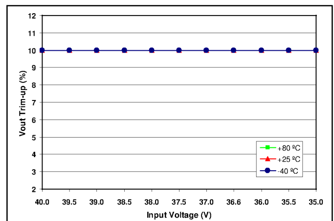
Figure 18: Maximum trim up vs. input voltage at different temperatures V_{in}=35.0\sim 40.0\ \text{V} .
