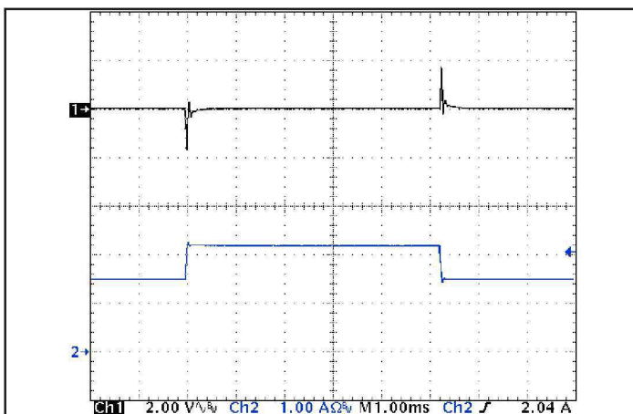
Figure 5: Output voltage response to step-change in load current (50%-75%-50% of Iout(max); dI/dt = 0.1A/μs). Load cap: 1μF ceramic cap. Ch 1: Vout, Ch 2: Iout.
