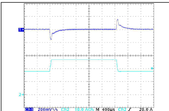
Figure 5: Output voltage response to step-change in load current (50%-75%-50% of Iout(max); di/dt = 0.1A/\mu s ). Load cap: 15µF tantalum cap and 1µF ceramic cap. Ch 1: Vout, Ch 2: Iout.
