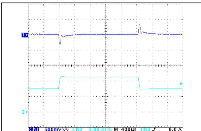
Figure 5: Output voltage response to step-change in load current (50%-75%-50% of I out (max); dI/dt = 0.1A/µs). Load cap: 15µF tantalum cap and 1µF ceramic cap. Ch 1: V out , Ch 2: I out .
