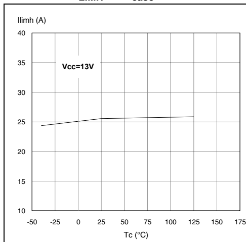
Figure 27. I_{LIMH} vs T_{case}
