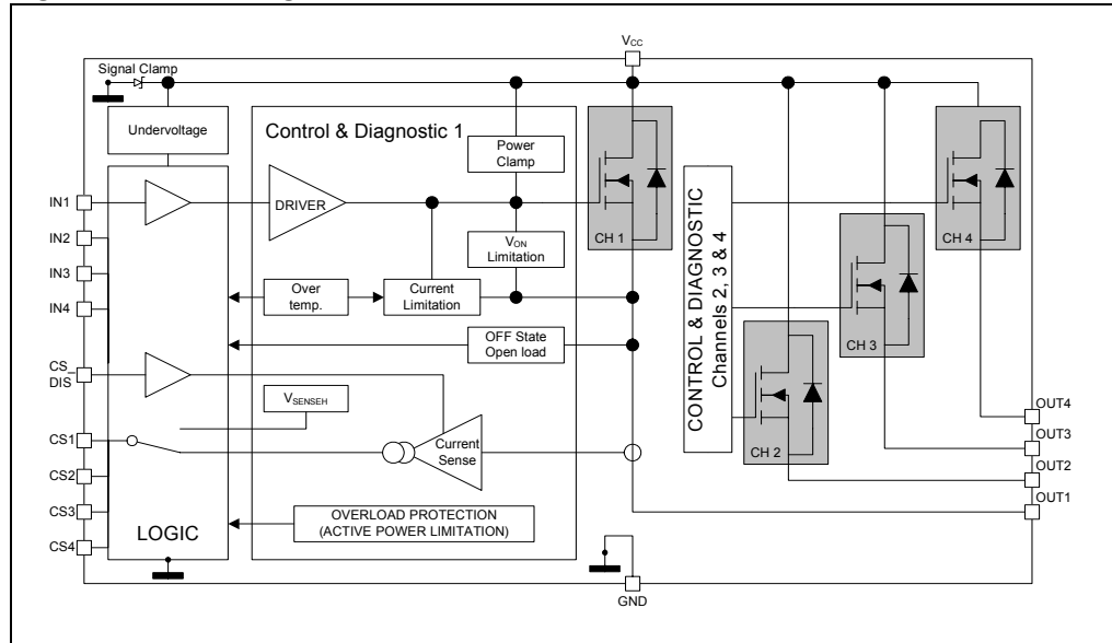
Figure 1. Block diagram
