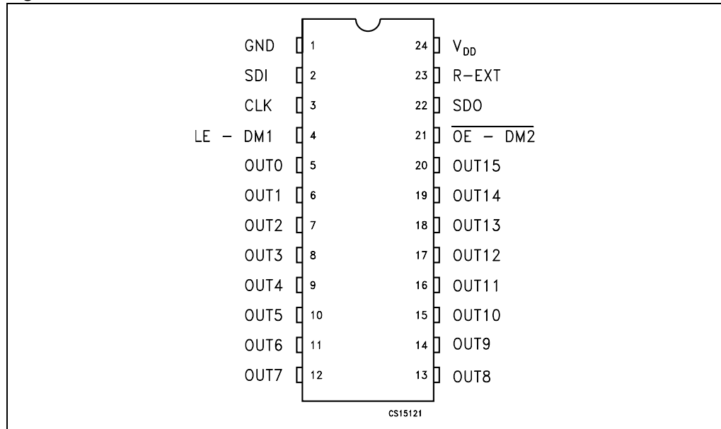
Figure 1. Pin connection
