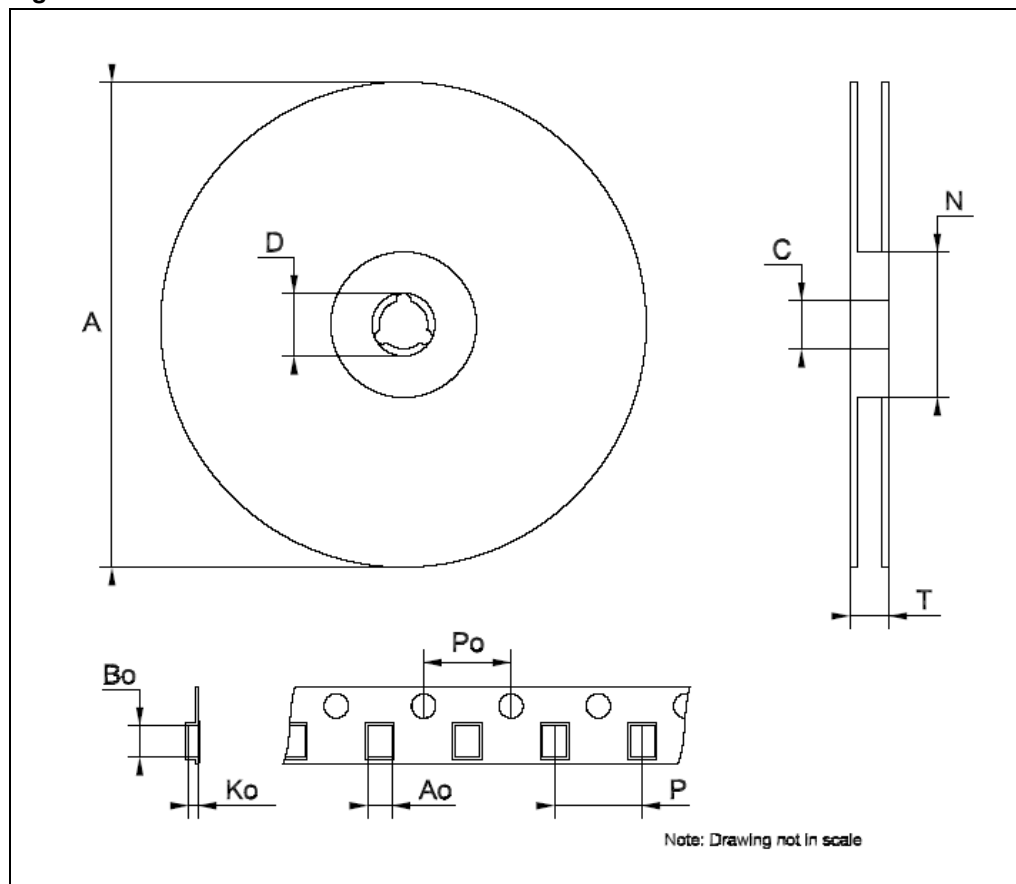
Figure 25. Reel dimensions
