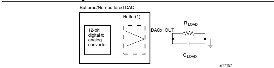
Figure 54. 12-bit buffered /non-buffered DAC
