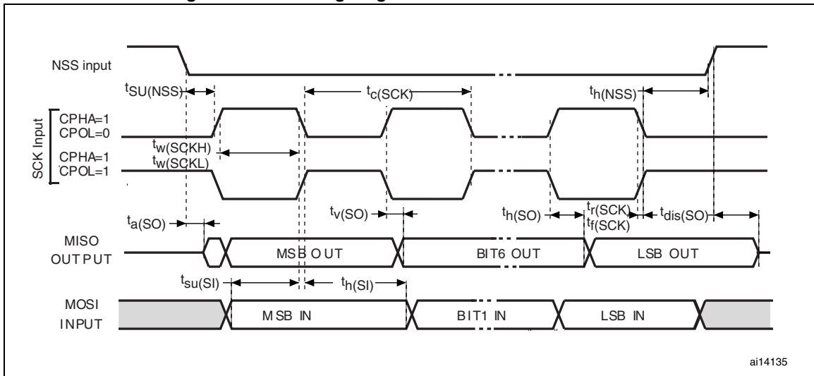
Figure 41. SPI timing diagram - slave mode and CPHA = 1
