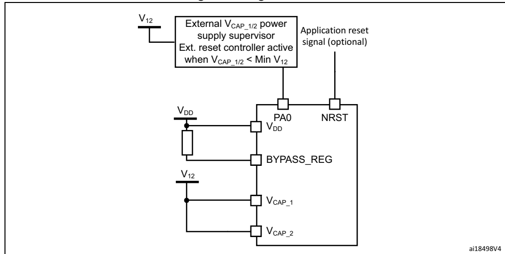
Figure 9. Regulator OFF
