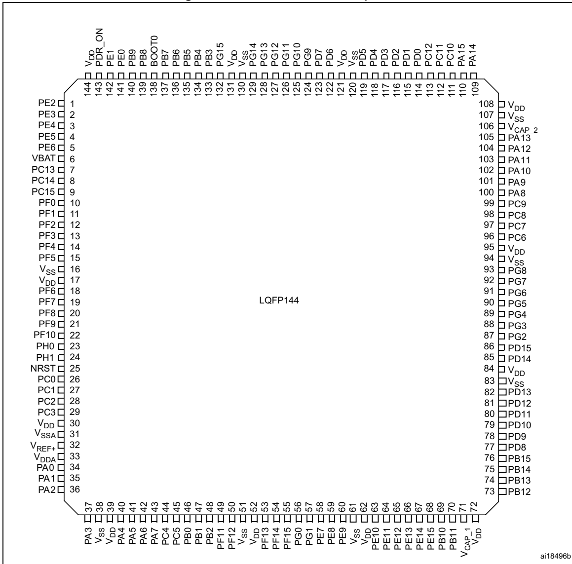
Figure 14. STM32F41x LQFP144 pinout
