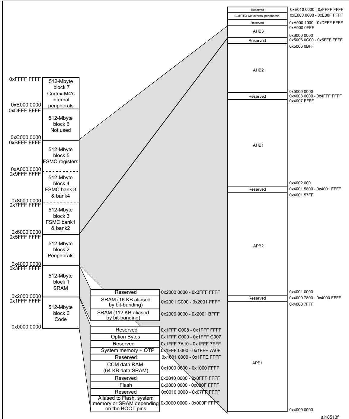
Figure 18. STM32F41x memory map
