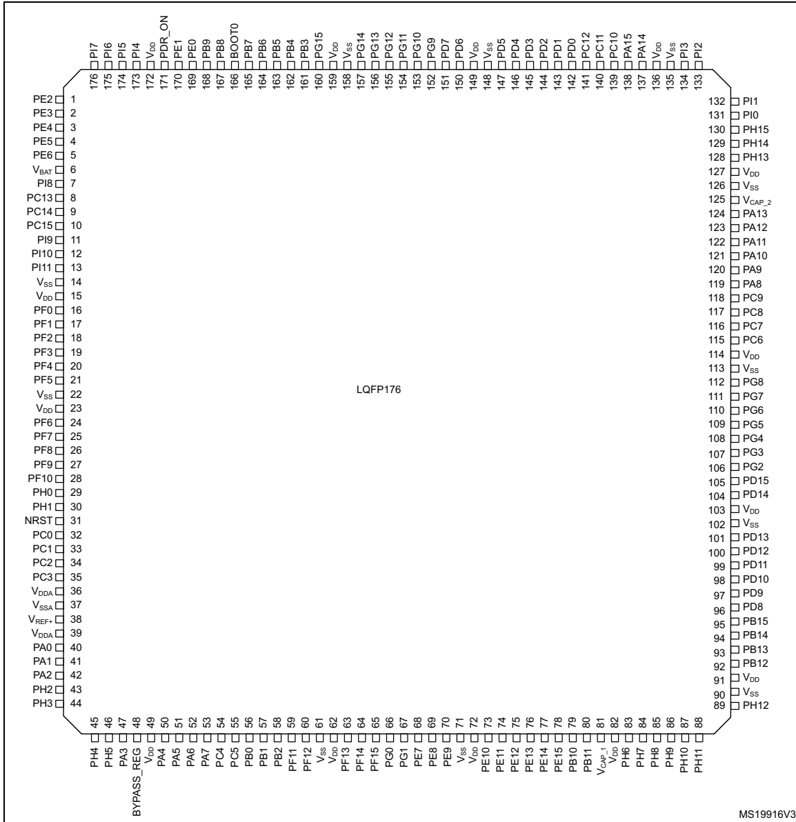
Figure 15. STM32F41x LQFP176 pinout
