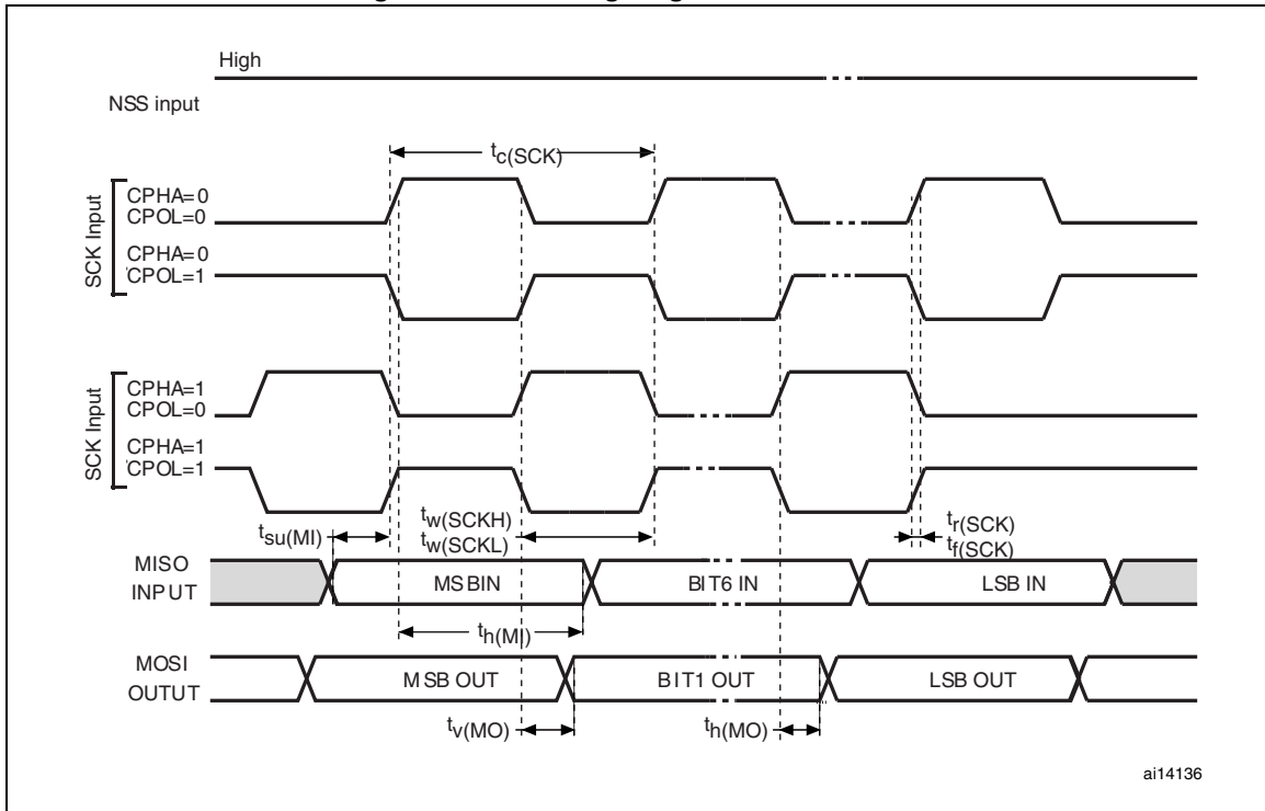
Figure 42. SPI timing diagram - master mode
