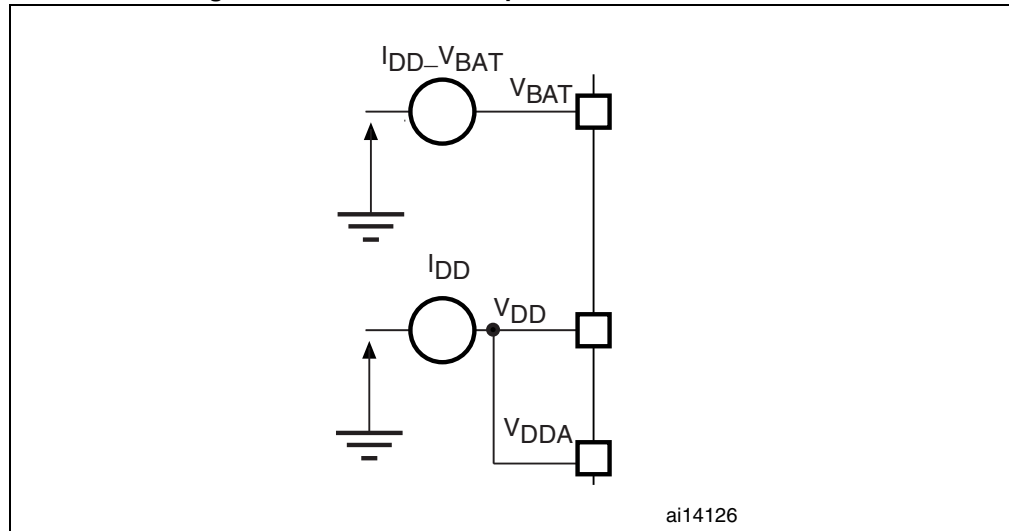
Figure 22. Current consumption measurement scheme
