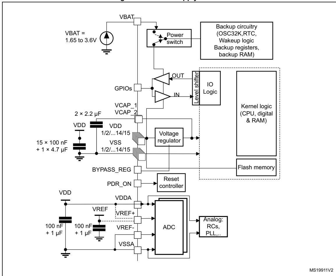
Figure 21. Power supply scheme
