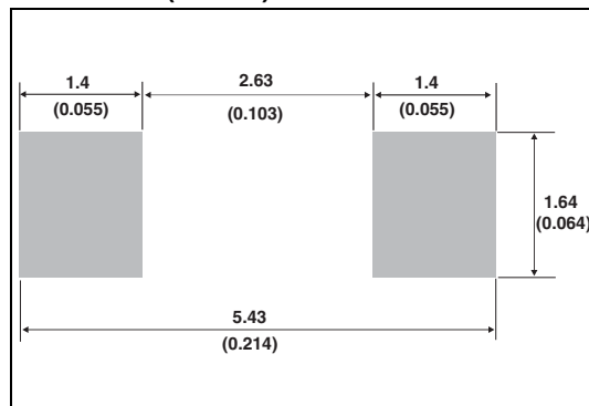
Figure 13. Footprint dimensions in mm (inches)
