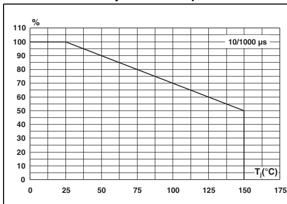
Figure 3. Peak power dissipation versus initial junction temperature
