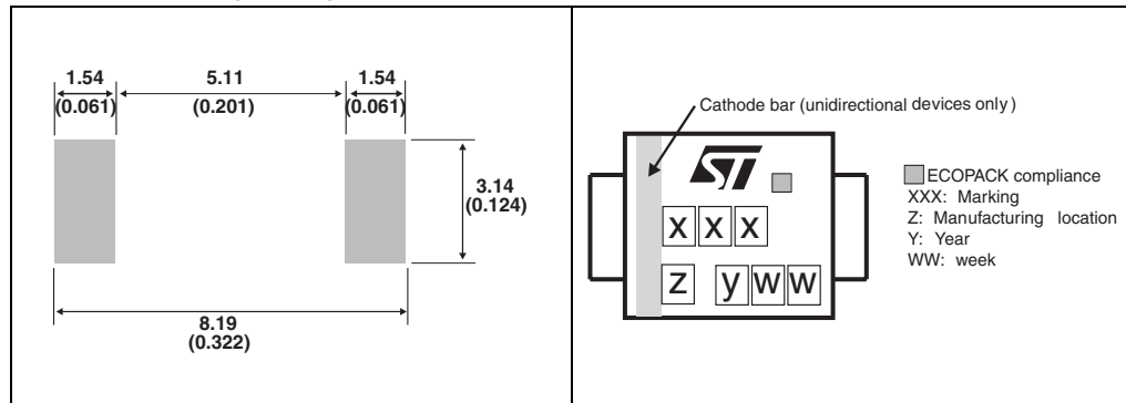
Figure 17. SMC footprint dimensions in mm (inches) Figure 18. Marking layout (1)
