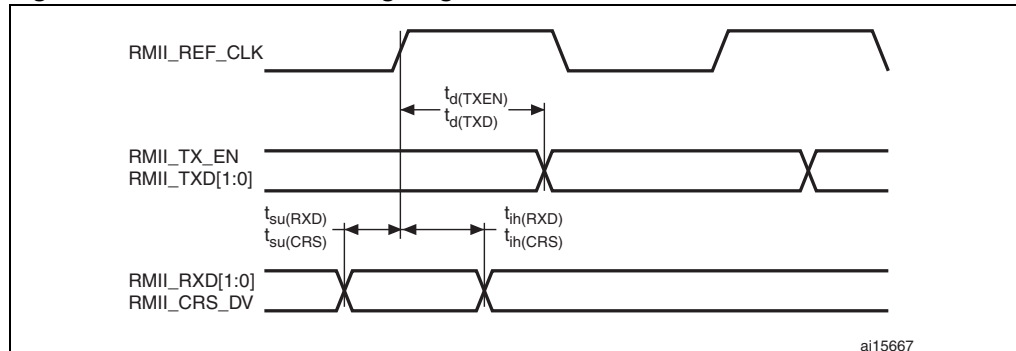
Figure 45. Ethernet RMII timing diagram
