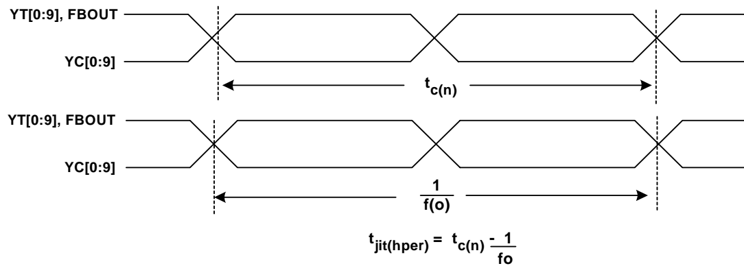
Figure 4. Period Jitter
