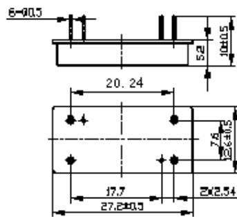
Package Outline
