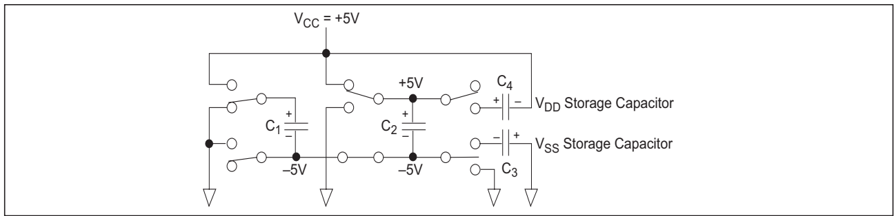
Figure 14. Charge Pump — Phase 1
