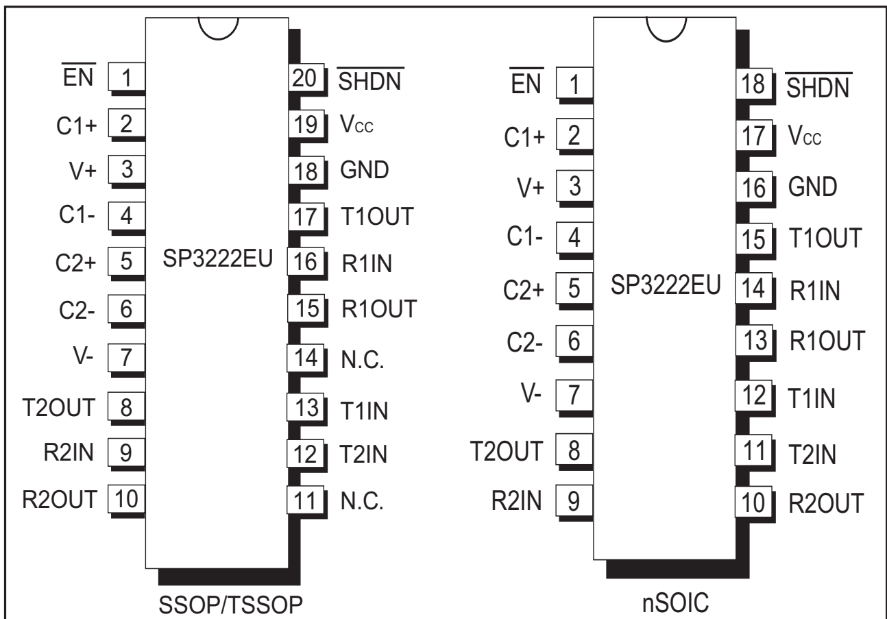
Figure 7. Pinout Configurations for the SP3222EU
