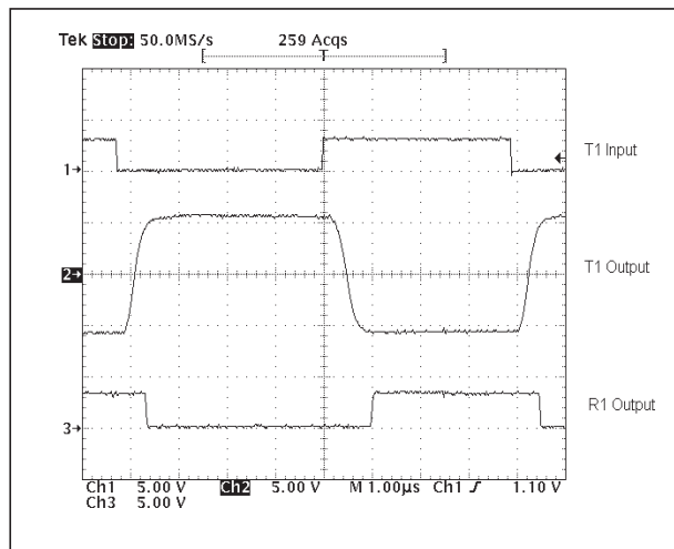
Figure 12. Loopback Test results at 250kbps
