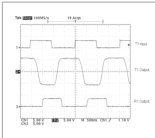
Figure 13. Loopback Test results at 1000Kbps
