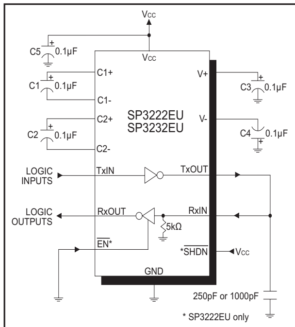
Figure 11. SP3222EU/SP3232EU Driver Loopback Test Circuit
