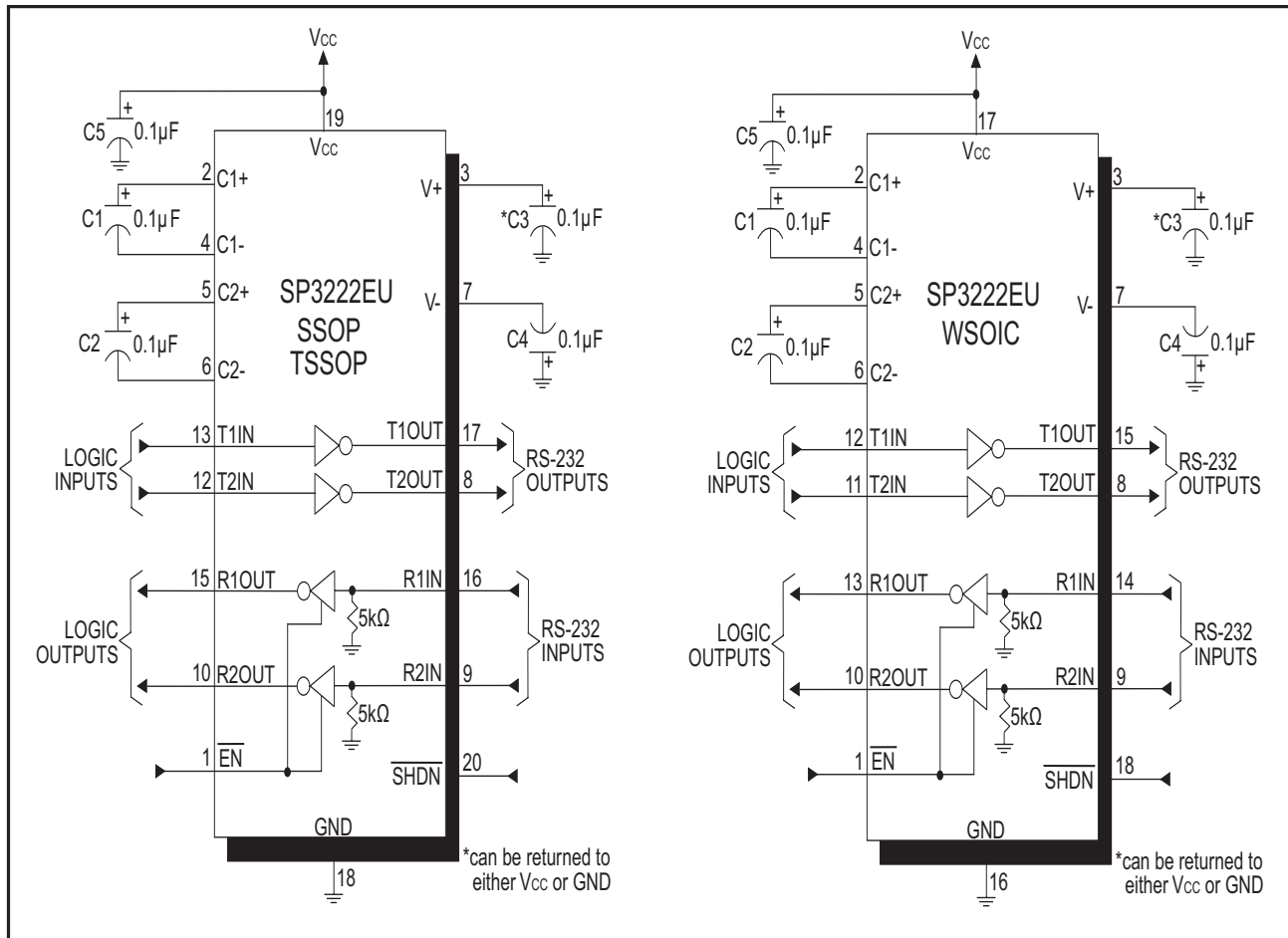
Figure 9. SP3222EU Typical Operating Circuits
