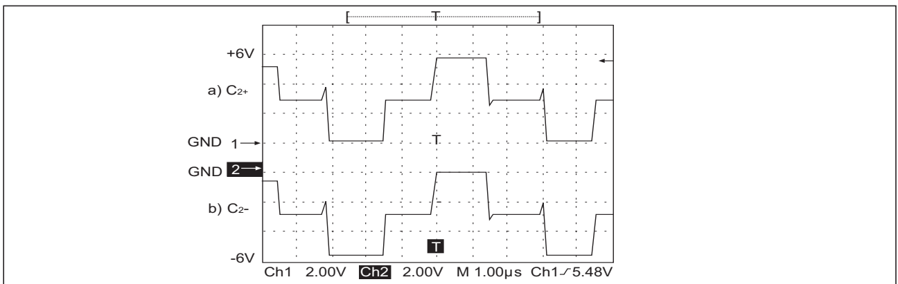
Figure 16. Charge Pump Waveforms
