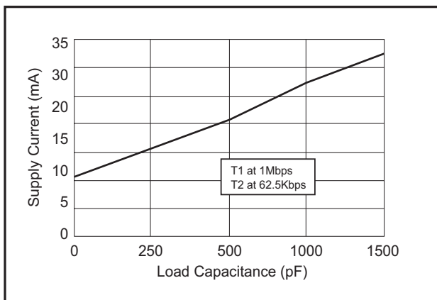
Figure 3. Supply Current VS. Load Capacitance when Transmitting Data for the SP3222EU and SP3232EU
