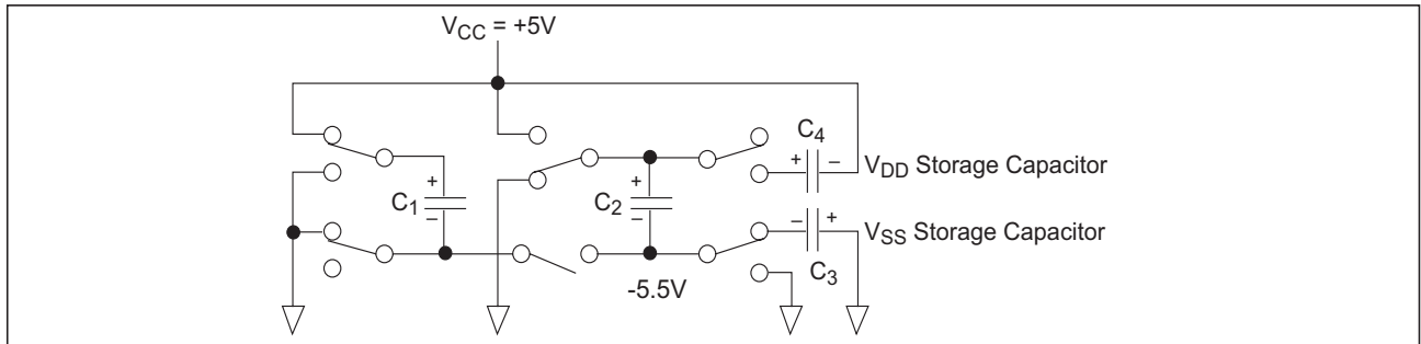
Figure 15. Charge Pump — Phase 2
