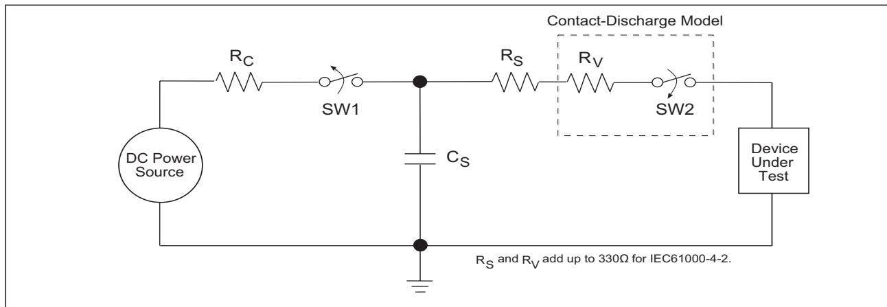
Figure 20. ESD Test Circuit for IEC61000-4-2
