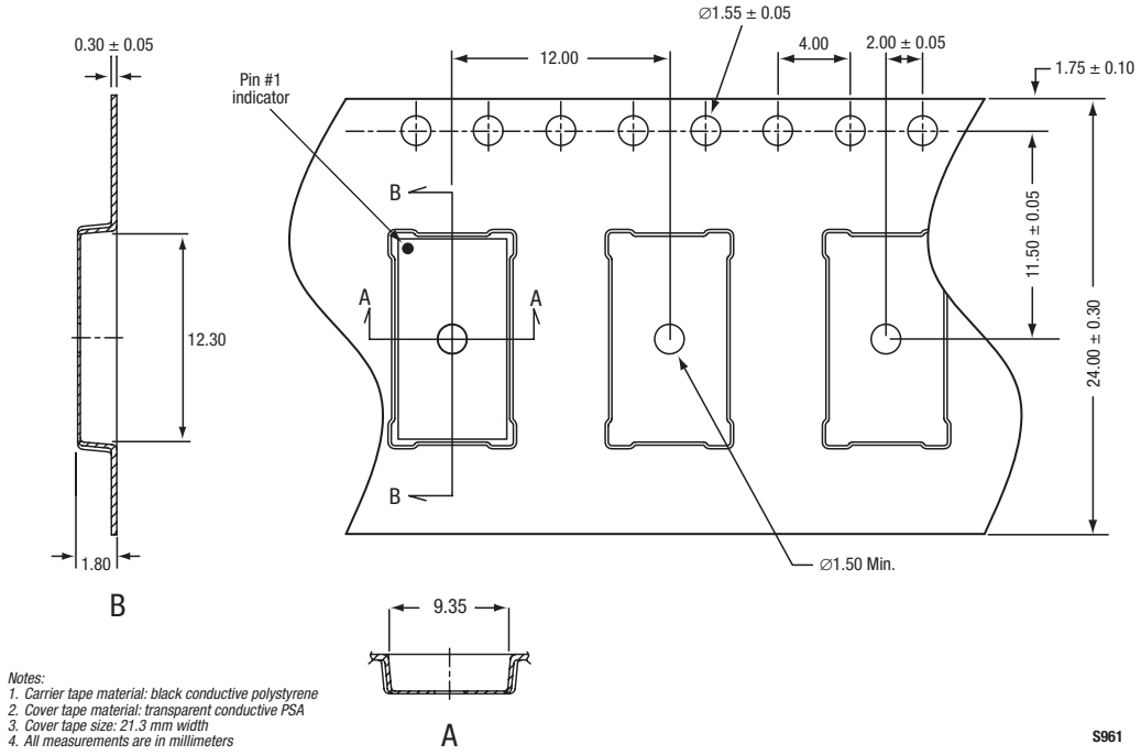
Figure 9. SKY73121 Tape and Reel Dimensions
