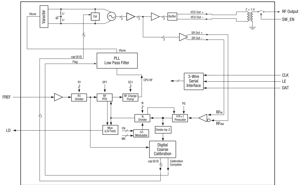
Figure 2. SKY73121 Functional Block Diagram
