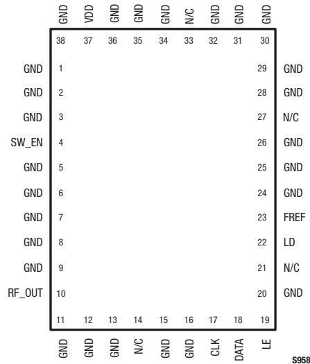
Figure 1. SKY73121 Pinout– 38-Pin MCM Package (Top View)
