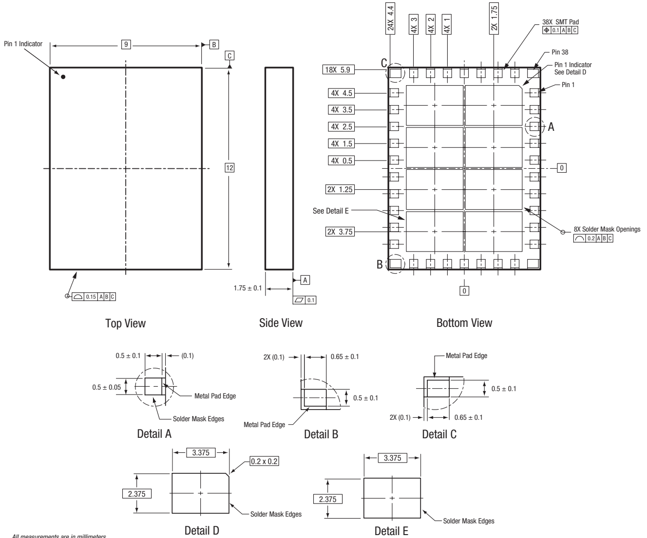
Figure 8. SKY73121 38-Pin MCM Package Dimensions
