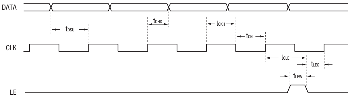
Figure 3. SKY73121 Serial Data Input Timing Diagram (MSB First)
