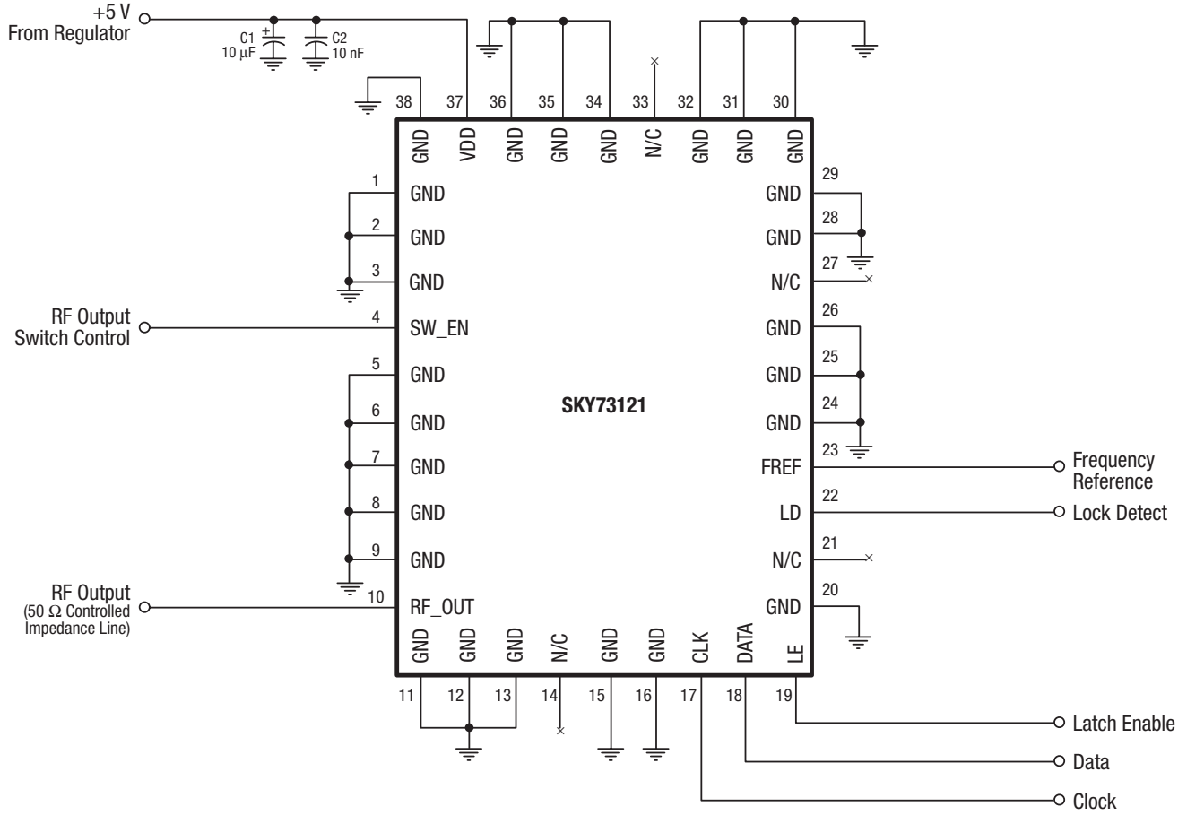
Figure 7. SKY73121 Typical Application Schematic
