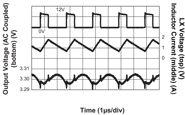
Step-Down Converter Output Ripple ( V_{IN} = 12V ; V_{OUT} = 3.3V ; I_{OUT} = 1.2A )
