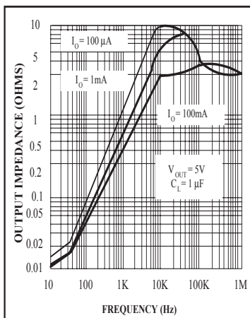
Output Impedance
