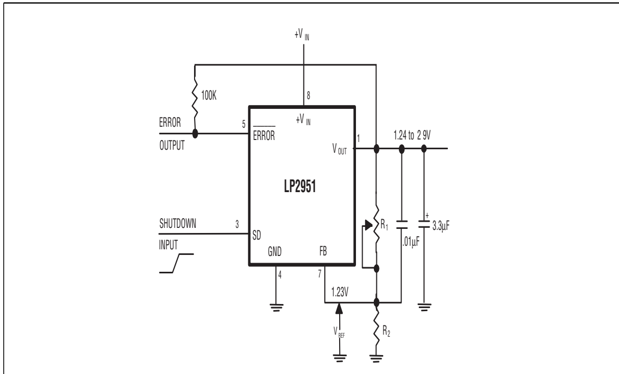
Figure 2. Adjustable Regulator
