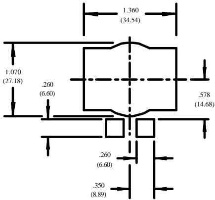
SUGGESTED PCB FOOTPRINT IN (mm)
