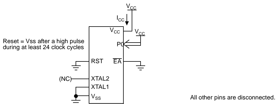
Figure 5. I_{CC} Test Condition, Power-down Mode
