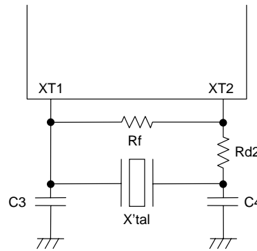
Figure 2 Crystal Oscillator Circuit
