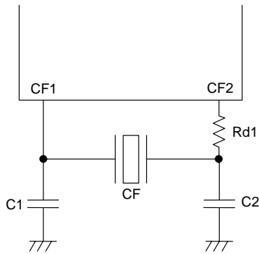
Figure 1 Ceramic Oscillator Circuit
