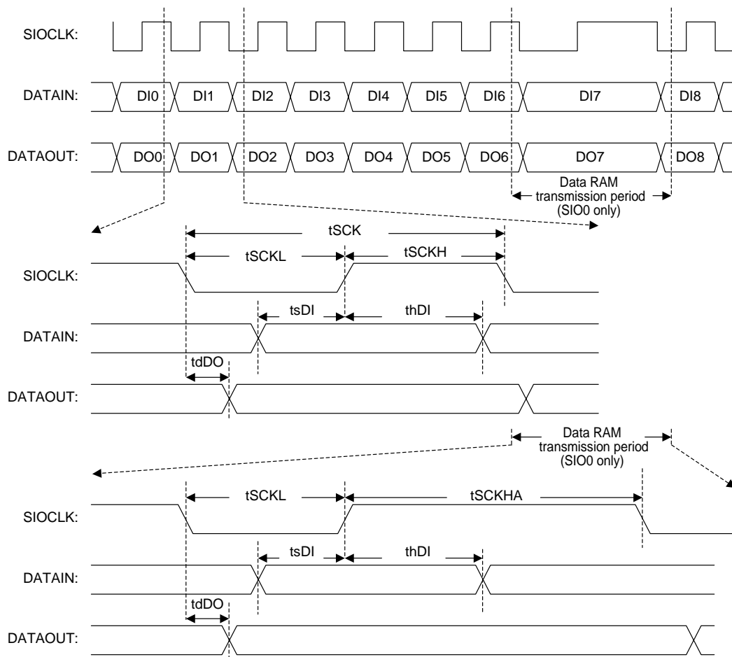
Figure 6 Serial Input/Output Wave Form
