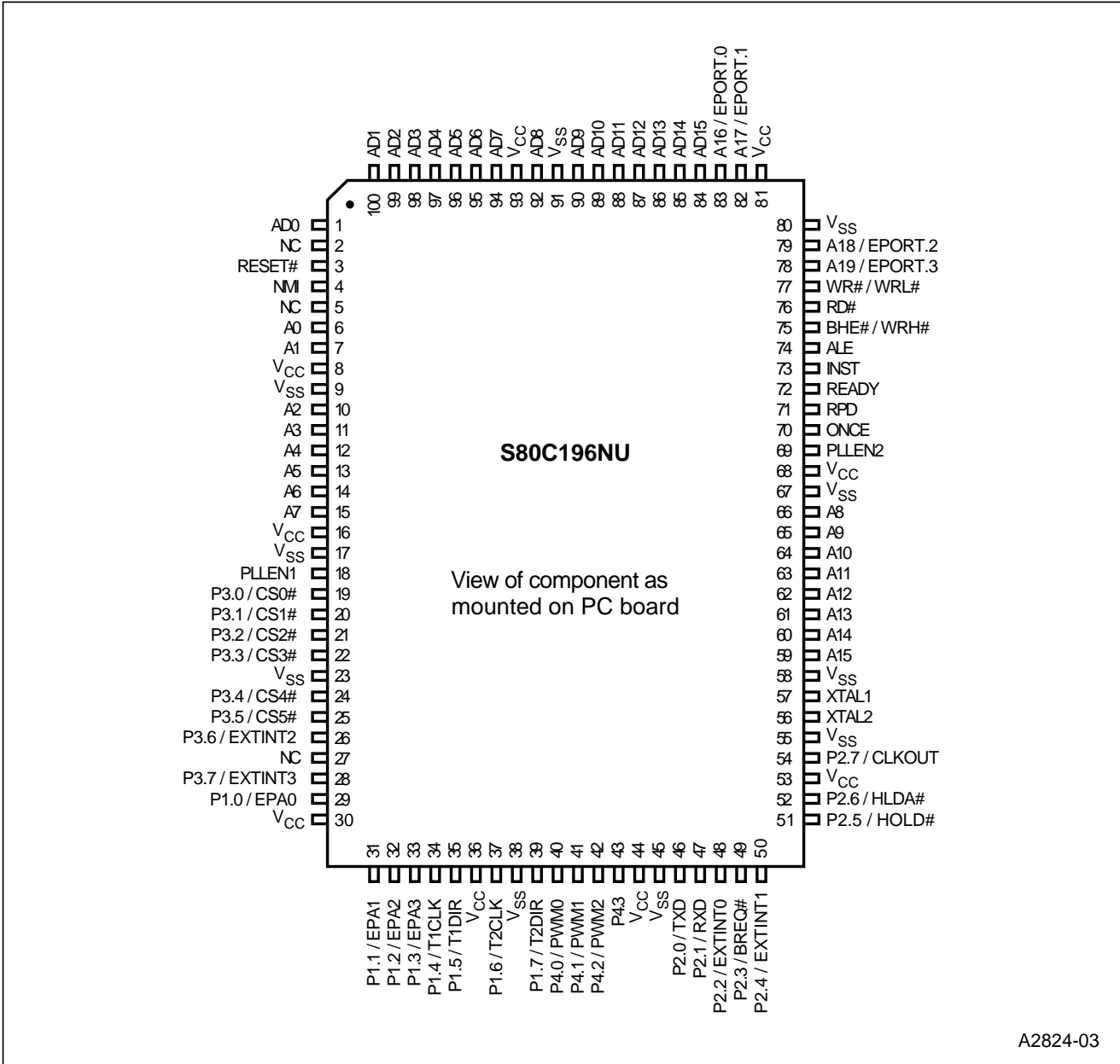
Figure 4. 80C196NU 100-pin QFP Package
