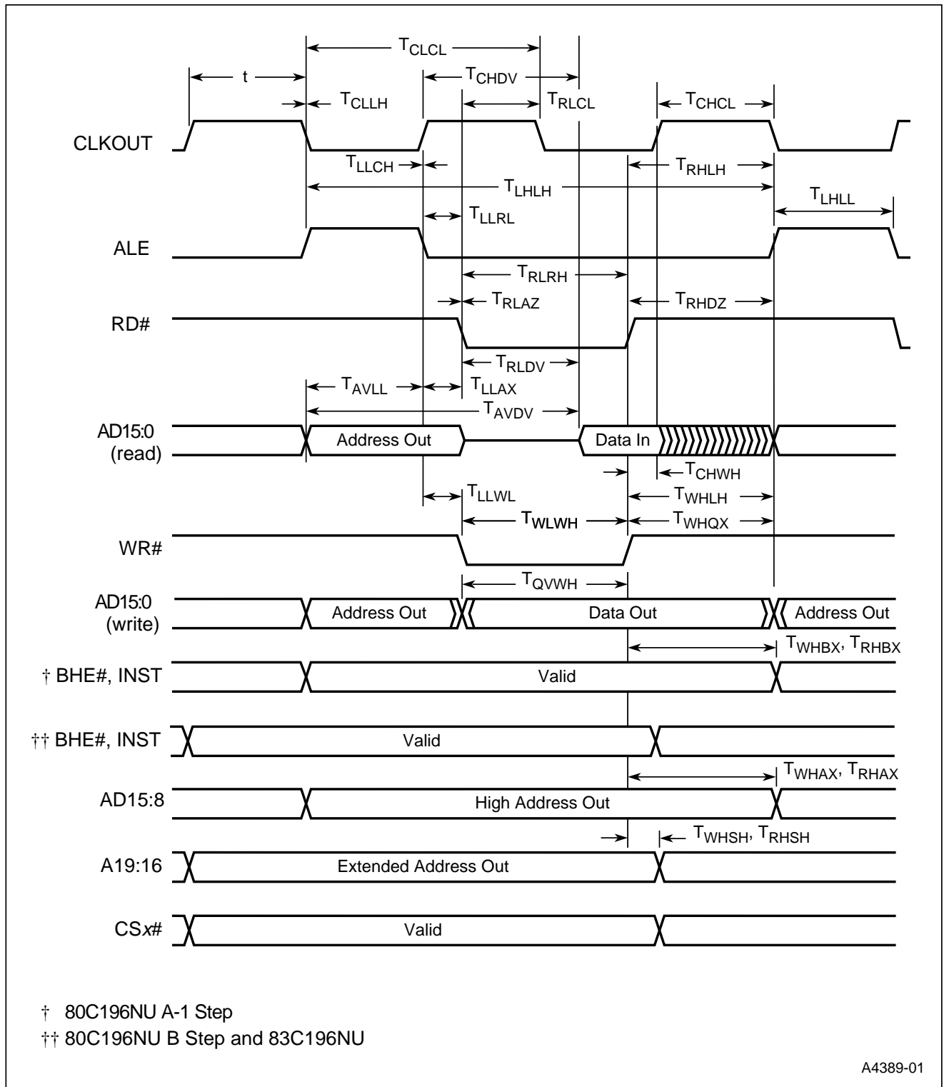
Figure 7. System Bus Timings, Multiplexed Bus Mode
