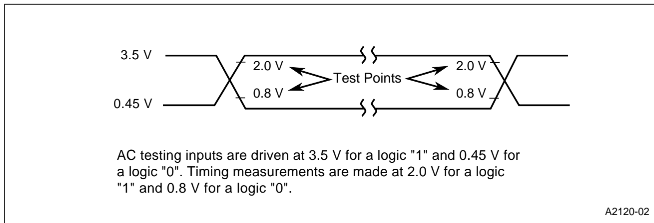
Figure 15. AC Testing Output Waveforms During 5.0 Volt Testing
