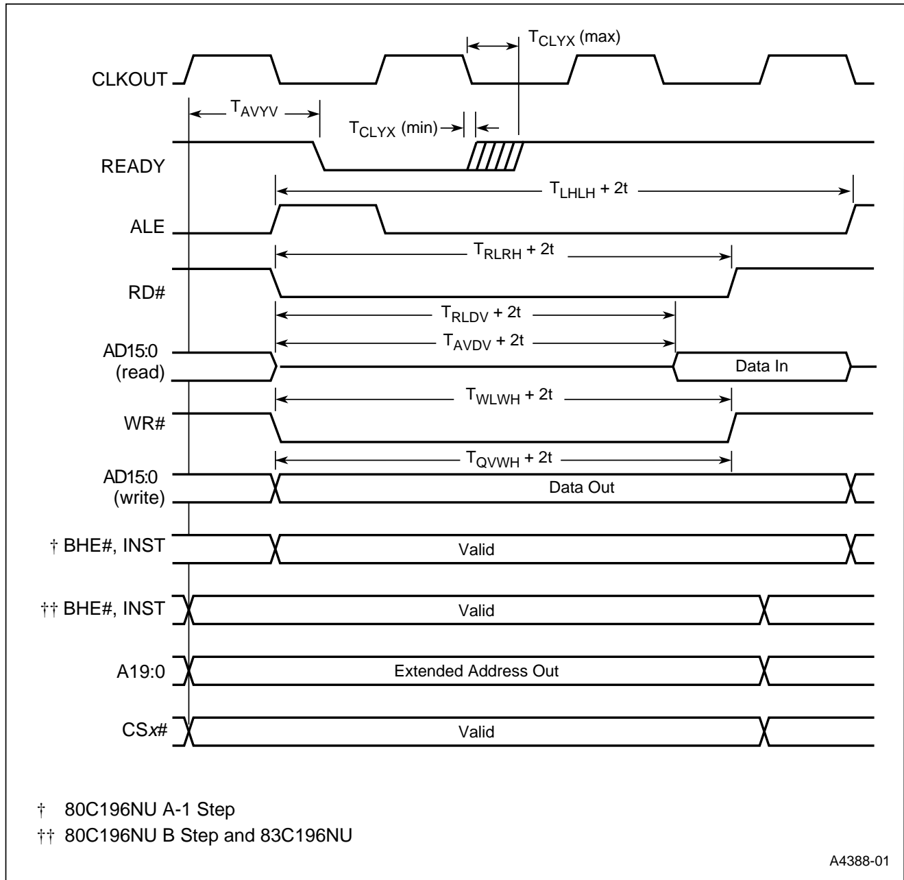
Figure 8. READY Timing, Multiplexed Bus Mode
