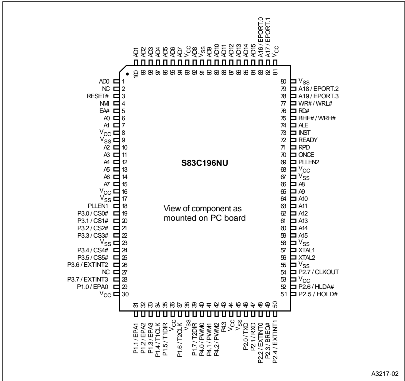
Figure 5. 83C196NU 100-pin QFP Package
