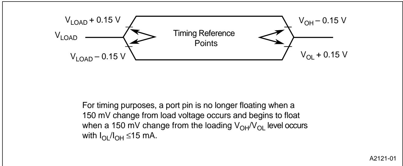
Figure 16. Float Waveforms During 5.0 Volt Testing
