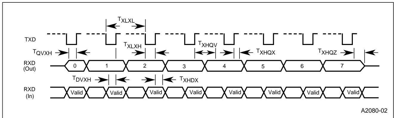
Figure 13. Serial Port Waveform — Synchronous Mode 0
