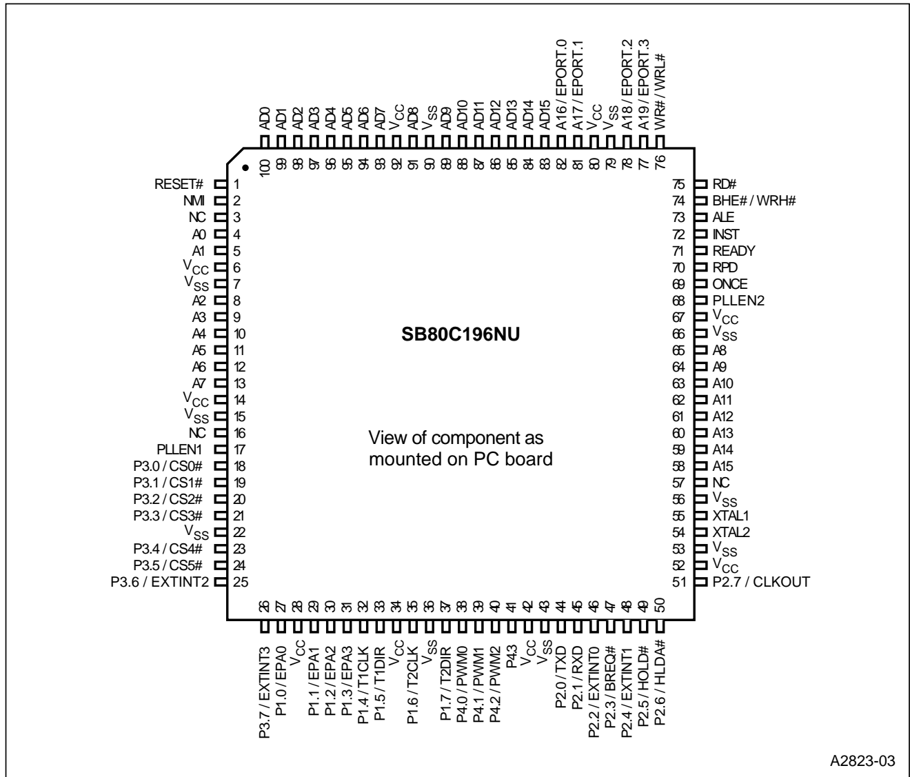
Figure 3. 80C196NU 100-pin SQFP Package
