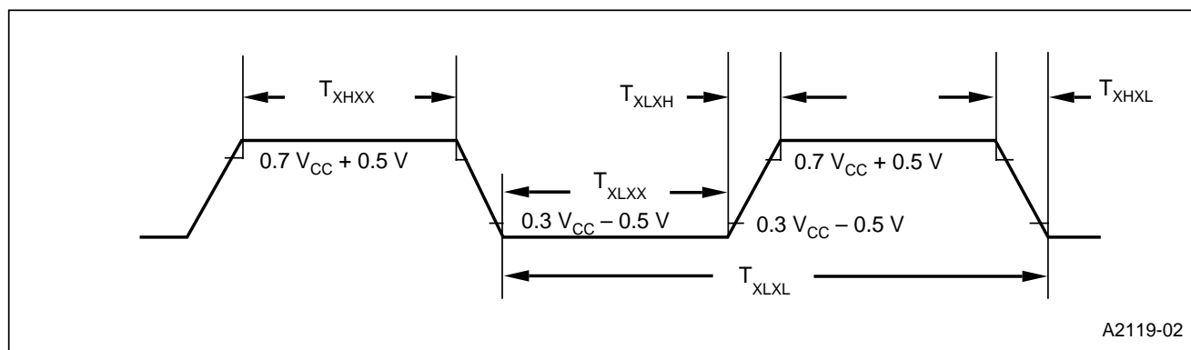
Figure 14. External Clock Drive Waveforms
