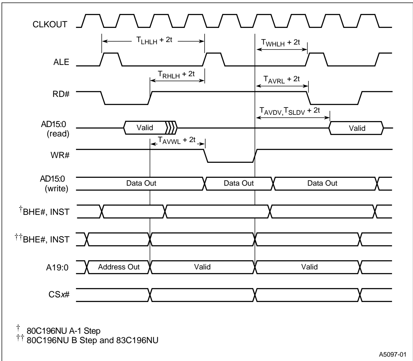
Figure 11. Deferred Bus Mode Timing Diagram
