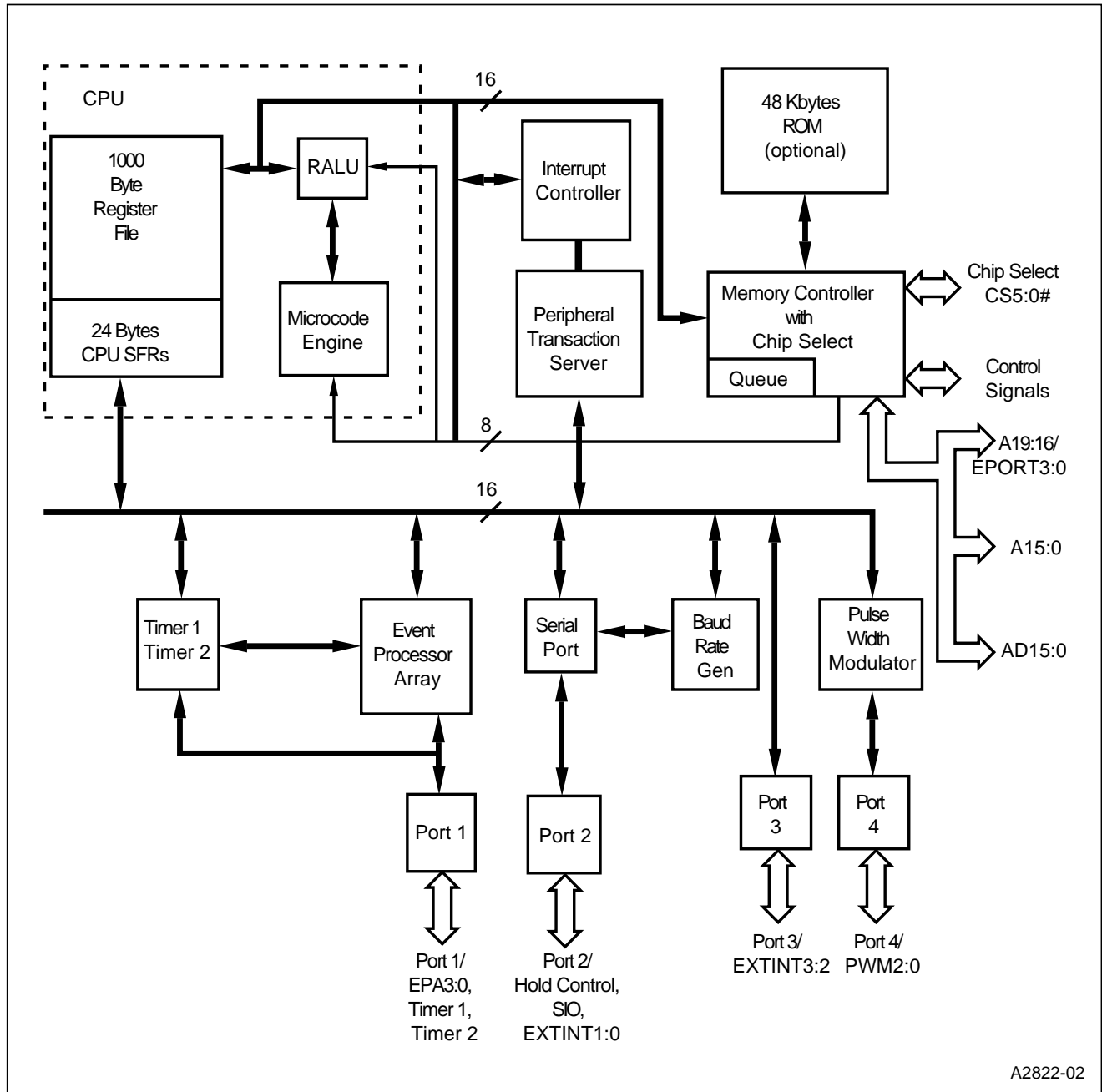
Figure 1. 8XC196NU Block Diagram
