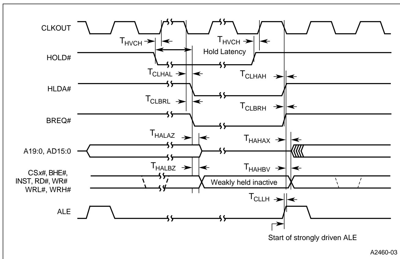
Figure 12. HOLD#, HLDA# Timing Diagram
