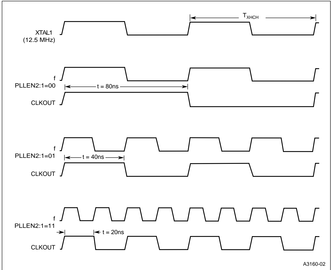
Figure 6. Effect of Clock Mode on CLKOUT
