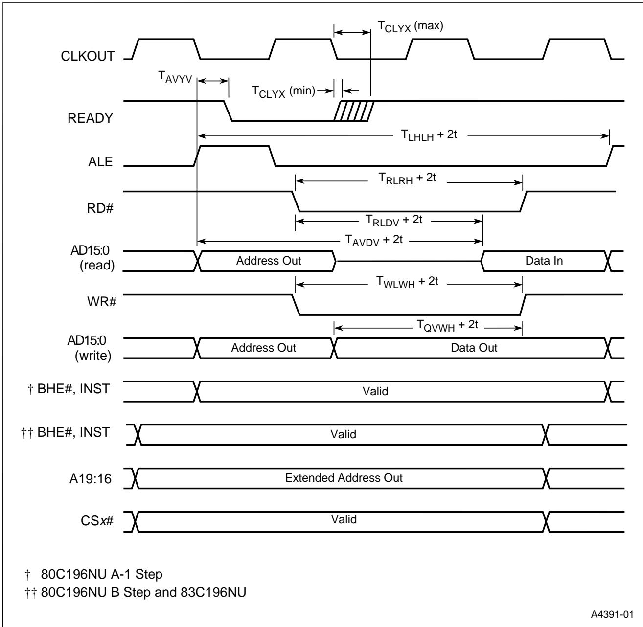
Figure 10. READY Timing, Demultiplexed Bus Mode
