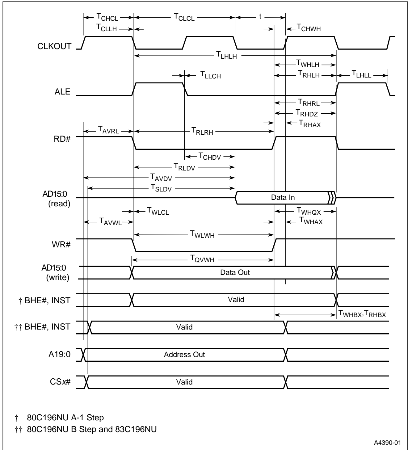
Figure 9. System Bus Timings, Demultiplexed Bus Mode
