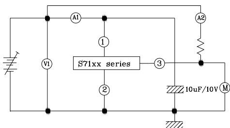
Test Circuit 1
