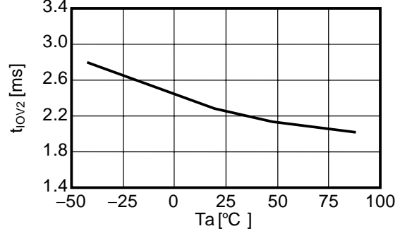
Overcurrent 2 detection delay time vs. temperature
