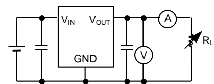
2. Output current - output voltage
