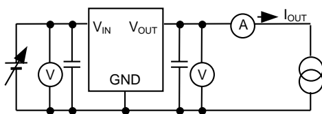
1. Input voltage - output voltage
