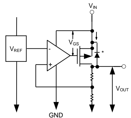
Figure 5 Error amplifier
