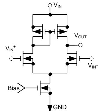
Figure 5 Error amplifier
