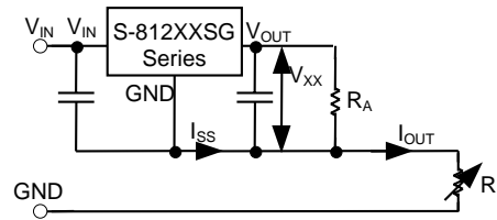
Figure 16 Constant current regulator
