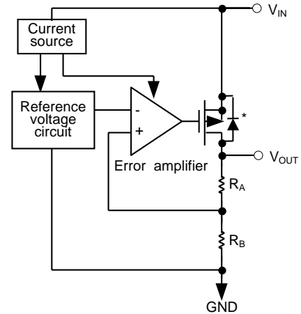
Figure 4 Reference block diagram
