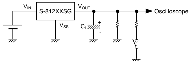
Figure 10 Measuring circuit
