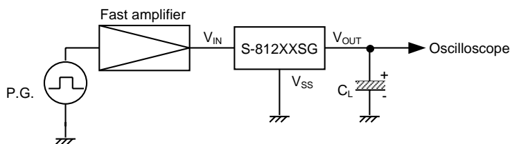
Figure 8 Measuring circuit
