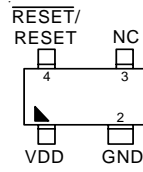
SC-82 (R-Type)
