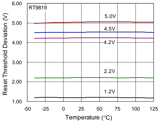
Reset Threshold Deviation vs. Temperature
