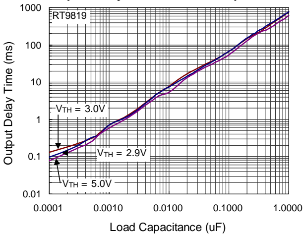
Output Delay Time vs. Load Capacitance
