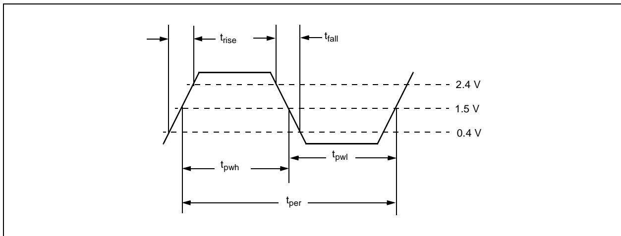
Figure 4-2. Output Waveform
