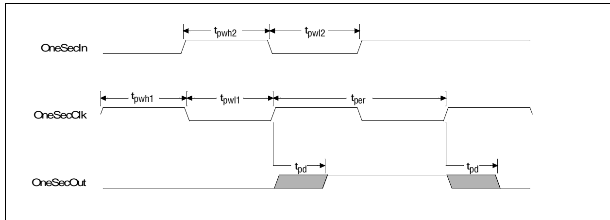
Figure 4-13. One-second Timing Diagram
