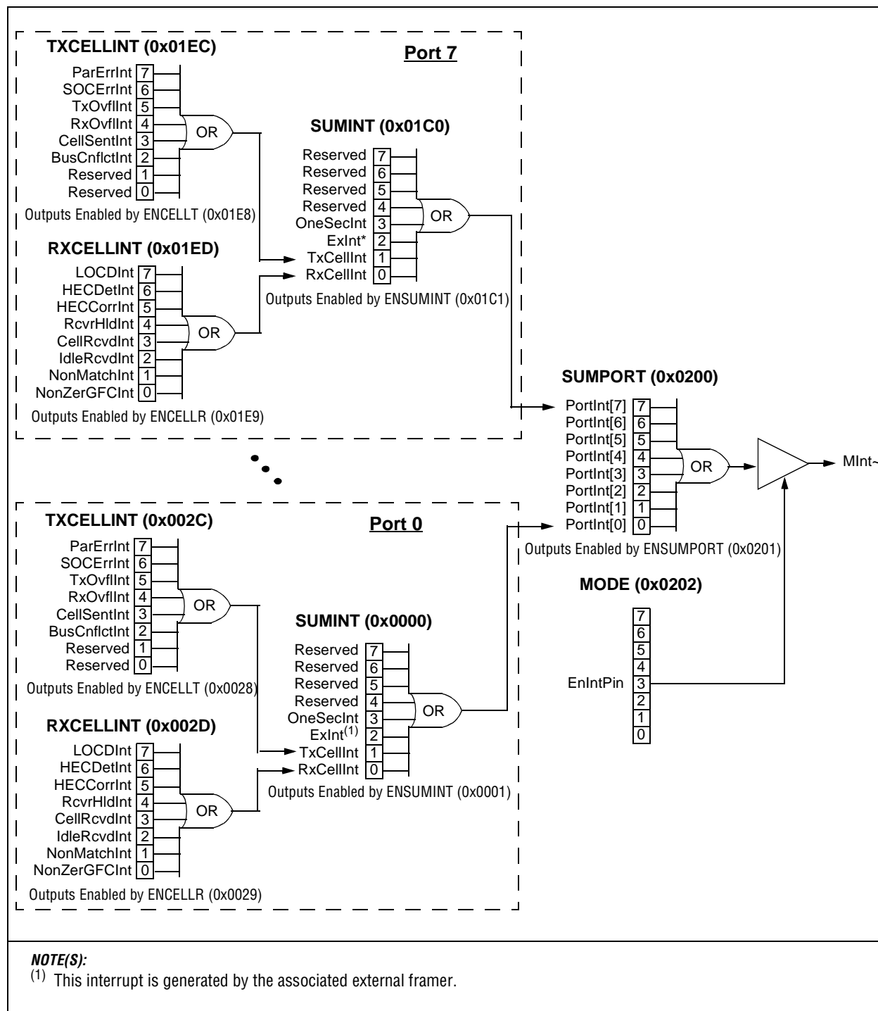
Figure 2-11. Interrupt Indication Diagram
