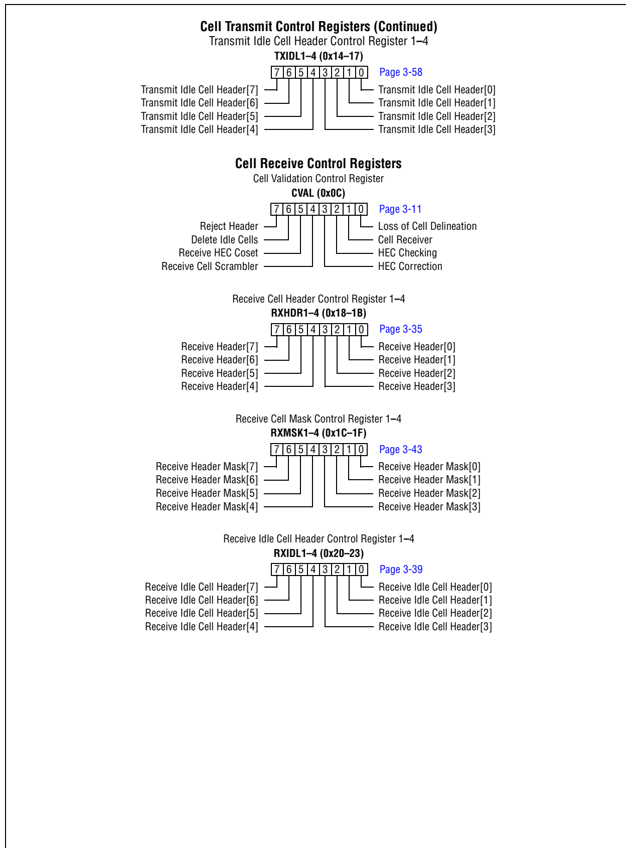
Figure C-1. Register Summary (3 of 8)
