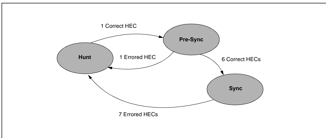
Figure 2-1. Cell Delineation Process
